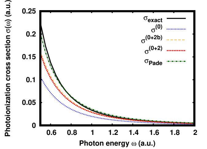
Fig. 1. Photoionization cross section of the hydrogen atom ( Z = 1 ). The exact cross section \sigma_{\text{exact}}(\omega) [Eq. (46)] is compared with the zeroth-order semiclassical approximation \sigma^{(0)}(\omega) [Eq. (42)], the partial second-order semiclassical approximation \sigma^{(0+2b)}(\omega) = \sigma^{(0)}(\omega) + \sigma^{(2b)}(\omega) [Eqs. (42) and (44)], the full second-order semiclassical approximation \sigma^{(0+2)}(\omega) = \sigma^{(0)}(\omega) + \sigma^{(2b)}(\omega) + \sigma^{(2c)}(\omega) [Eqs. (42), (44), and (45)], and the Padé approximant \sigma_{\text{Padé}}(\omega) [Eq. (48)].
