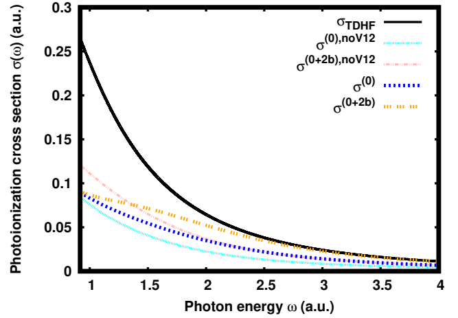
Fig. 3. Photoionization cross section of the helium atom ( Z = 2 ). The reference TDHF cross section \sigma_{\text{TDHF}}(\omega) [40, 9] is compared with the zeroth-order semiclassical cross section \sigma^{(0)}(\omega) [Eq. (60)] and the partial second-order semiclassical cross sections \sigma^{(0+2b)}(\omega) = \sigma^{(0)}(\omega) + \sigma^{(2b)}(\omega) [Eqs. (60) and (64)]. Also reported are the approximate zeroth-order and partial second-order semiclassical cross sections \sigma^{(0), \text{noV12}}(\omega) and \sigma^{(0+2b), \text{noV12}}(\omega) = \sigma^{(0), \text{noV12}}(\omega) + \sigma^{(2b), \text{noV12}}(\omega) [Eqs. (60) and (64)] in which the two-electron Coulomb interaction V_{12}(\mathbf{q}_1, \mathbf{q}_2) = 1/\|\mathbf{q}_1 - \mathbf{q}_2\| has been neglected.
