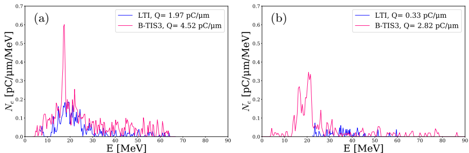
FIGURE 17. Energy spectrum of the accelerated electrons after a propagation of (a) 570 \mu\text{m} and (b) 950 \mu\text{m} .
