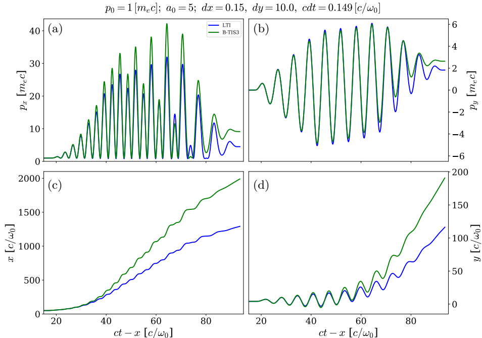
FIGURE 10. Evolution of the electron normalised momentum: (a) p_x , (b) p_y and normalised position: (c) x , (d) y with respect to the normalised coordinate ct - x for LTI and B-TIS3 with a transversely gaussian laser beam and an electron with an initial longitudinal momentum ( p_0 = m_e c )
