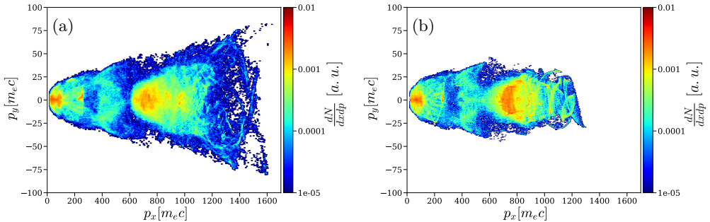
FIGURE 21. Phase space map (p_x, p_y) after 2.65 mm of laser propagation in the plasma: (a) LTI simulation, (b) B-TIS3 simulation.
