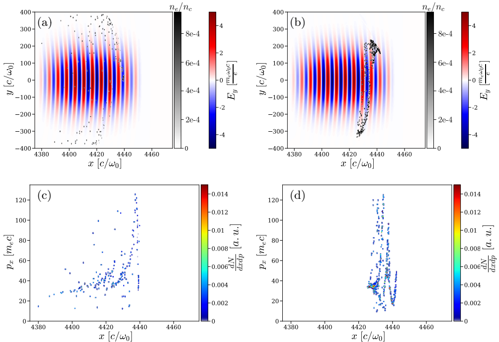
FIGURE 16. Top: electronic density map (greyscale) superimposed to the electric field E_y map (colours) after a propagation of 950 \mu\text{m} for (a) LTI and (b) B-TIS3. Bottom: phase space ( x, p_x ) after a propagation of 950 \mu\text{m} for (c) LTI and (d) B-TIS3.
