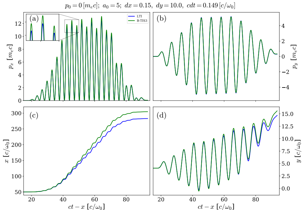
FIGURE 9. Evolution of the electron normalised momentum: (a) p_x , (b) p_y and normalised position: (c) x , (d) y with respect to the normalised coordinate ct - x for LTI and B-TIS3 with a transversely gaussian laser beam and an electron initially at rest ( p_0 = 0 ).
