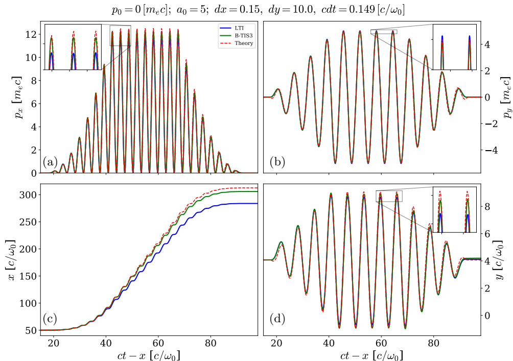
FIGURE 6. Evolution of the electron normalised momentum: (a) p_x , (b) p_y and normalised position: (c) x , (d) y with respect to the normalised coordinate ct - x for LTI and B-TIS3. The red dashed line shows the theoretical values expected from analytical model introduced earlier.
