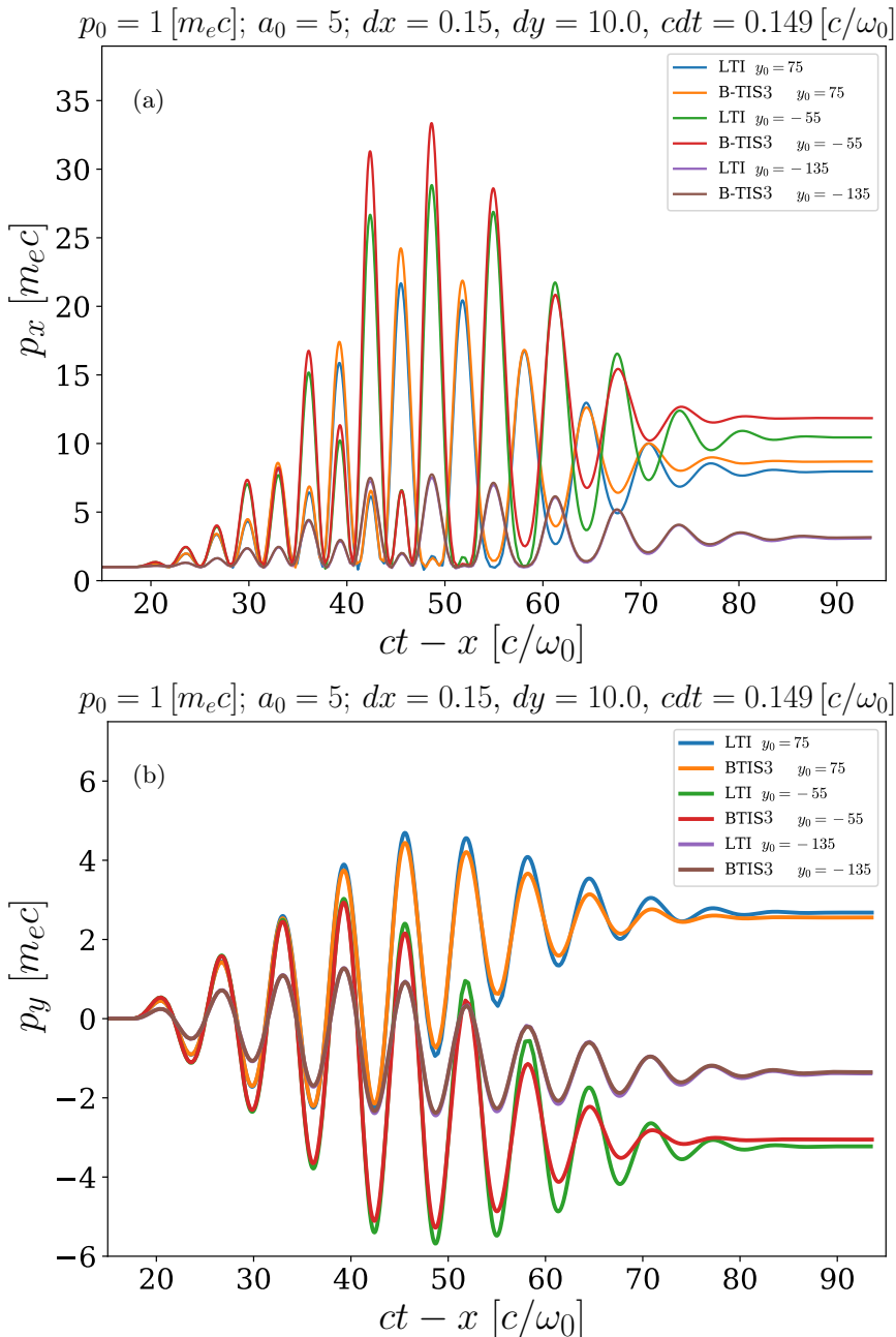
FIGURE 12. Evolution of the electron normalized momentum: (a) p_x , (b) p_y with respect to the normalised coordinate ct - x for LTI and B-TIS3, with p_0 = m_e c and varying initial transverse position y_0 of the electron. Note that the transverse profile of the laser is centered on y = 0 .
