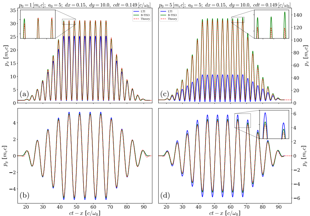
FIGURE 7. Evolution of the electron normalised momentum: (a) ( resp. (c)) p_x , (b) ( resp. (d)) p_y with respect to the normalised coordinate ct - x for LTI and B-TIS3 with p_0 = m_e c ( resp. p_0 = 5 m_e c ). The red dashed line shows the theoretical values expected from analytical model introduced earlier.
