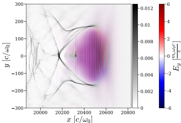
FIGURE 19. Electron density map normalised to the critical density n_c (greyscale) superimposed to the electric field E_y map.
