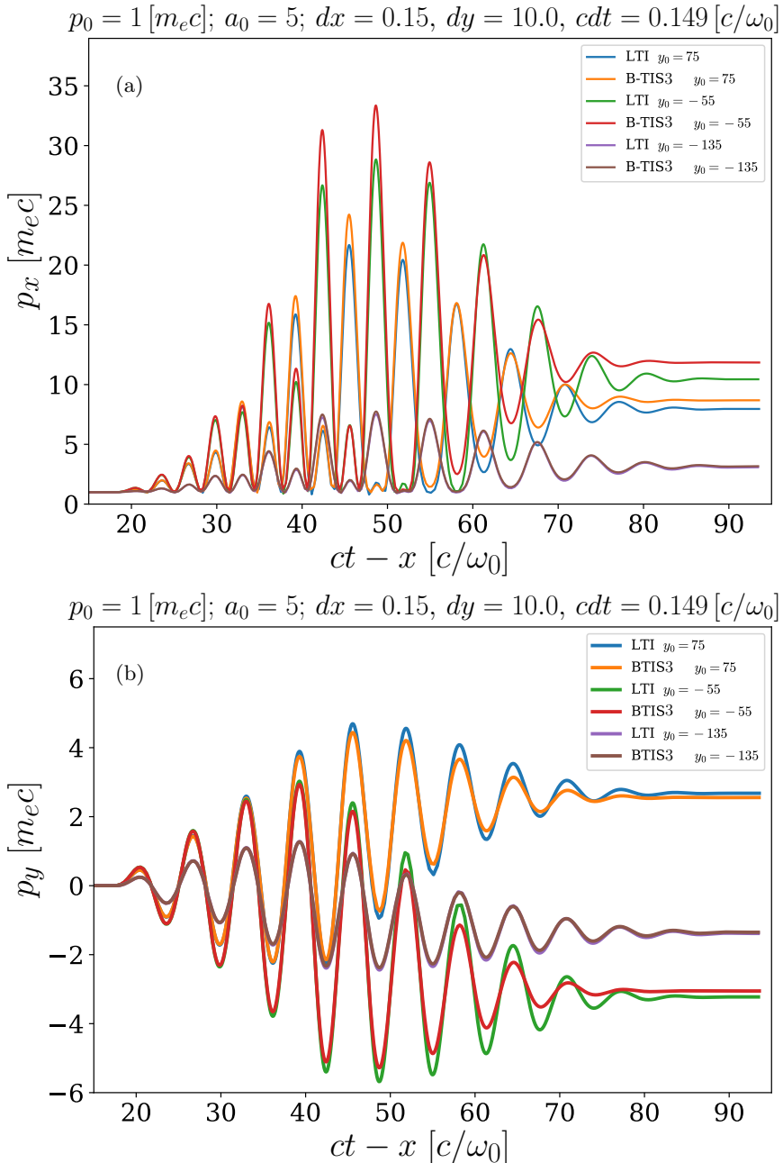
FIGURE 12. Evolution of the electron normalised momentum: (a) p_x , (b) p_y with respect to the normalised coordinate ct - x for LTI and B-TIS3, with p_0 = m_e c and varying initial transverse position y_0 of the electron. Note that the transverse profile of the laser is centered on y = 0 .
