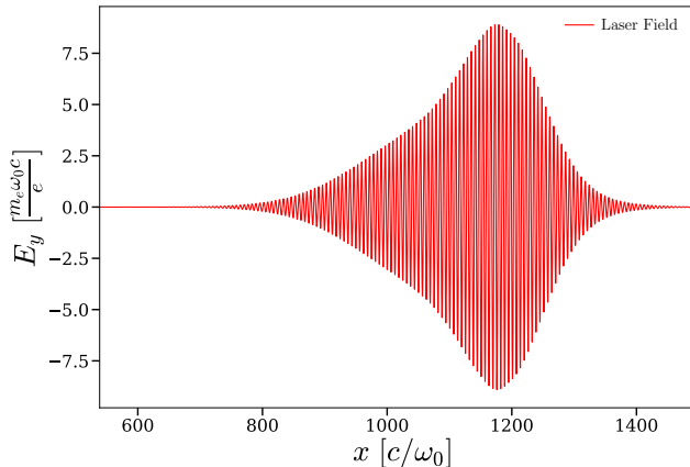
FIGURE 18. Temporal profile of the electric field E_y .
