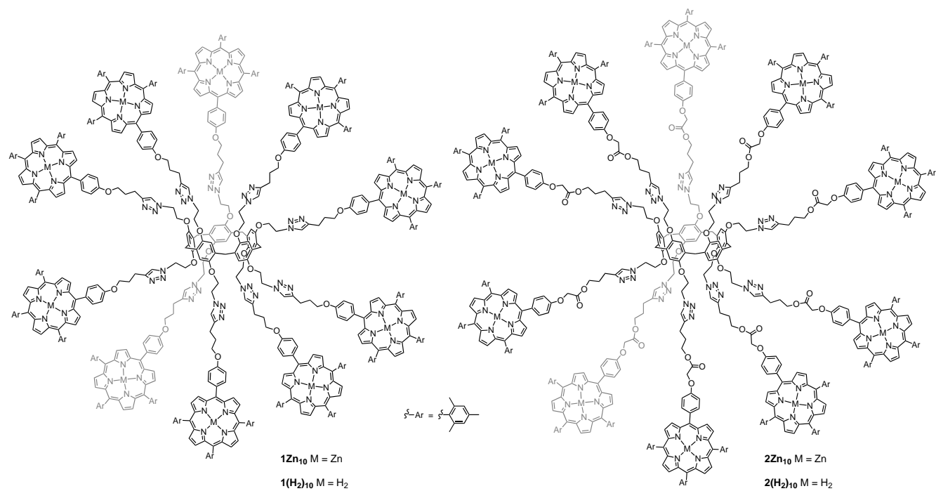
Figure 1. Multi-Zn(II)porphyrin arrays 1\text{Zn}_{10} and 2\text{Zn}_{10} as well as the corresponding free-base derivatives 1(\text{H}_2)_{10} and 2(\text{H}_2)_{10} .
