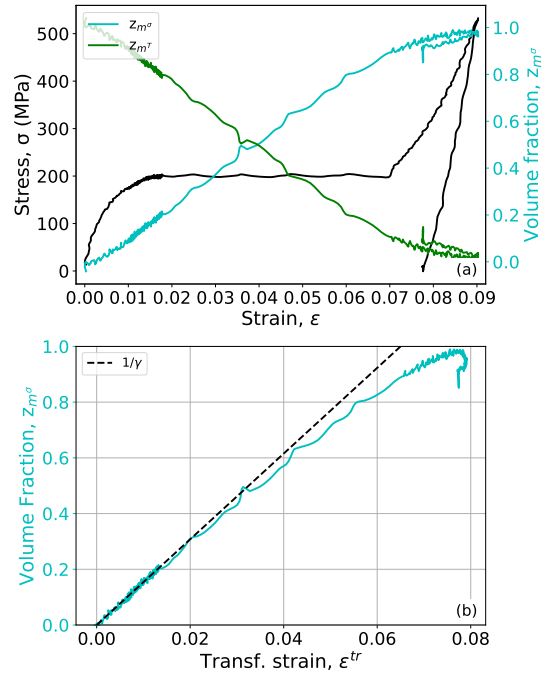
Figure 13: Stress\ volume fraction vs. strain (a) and volume fraction vs. transf. strain (b) for an isothermal loading at -40^\circ C - FW wire.
