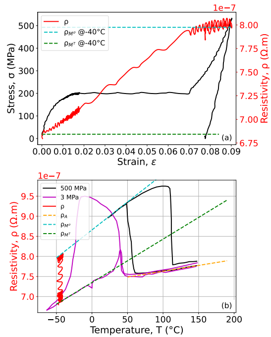
Figure 12: Stress\ resistivity vs. strain (a) and resistivity vs. temperature (b) for an isothermal loading at -40^\circ C - FW wire.
