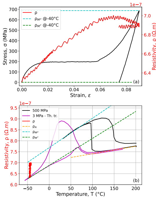
Figure 10: Stress\ resistivity vs. strain (a) and resistivity vs. temperature (b) for an isothermal loading at -40^\circ C - DN wire.
