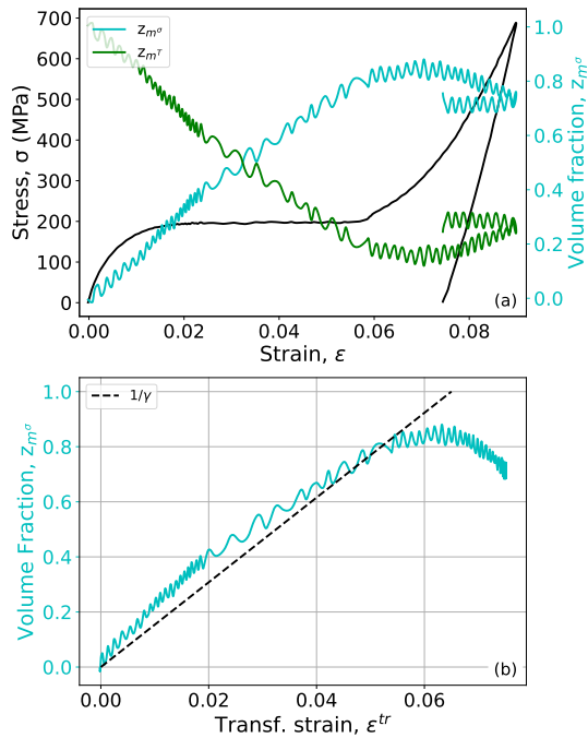
Figure 11: Stress\ volume fraction vs. strain (a) and volume fraction vs. transf. strain (b) for an isothermal loading at -40^\circ C - DN wire.
