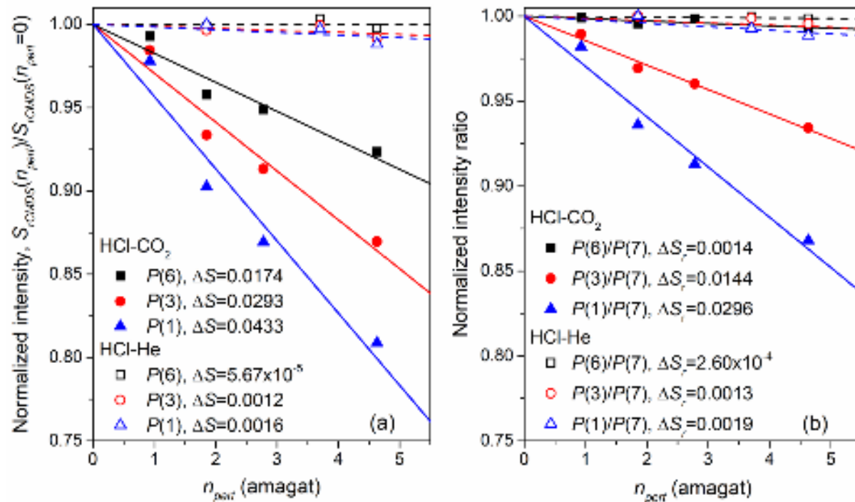
Figure 3: (a): Line intensity, S_{\text{rCMDS}} , retrieved from the rCMDS-calculated spectra vs the perturber density for the P(1) , P(3) and P(6) lines of HCl in \text{CO}_2 (full symbols) and in He (open symbols) and the corresponding linear fits. S_{\text{rCMDS}} were normalized to values at zero density S_{\text{rCMDS}}(n_{\text{pert}} = 0) (see text). (b): The same as for the left panel but normalized to the retrieved intensity of the P(7) line.
