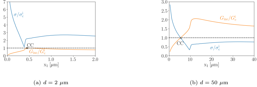
Figure 12: Application of the CC for \alpha = 90^\circ in the case of penetration, shown in Fig. 9, considering K_{IC}^a = 2 \text{ MPa} \cdot \text{m}^{1/2} and \sigma_c^a = 300 \text{ MPa} .
