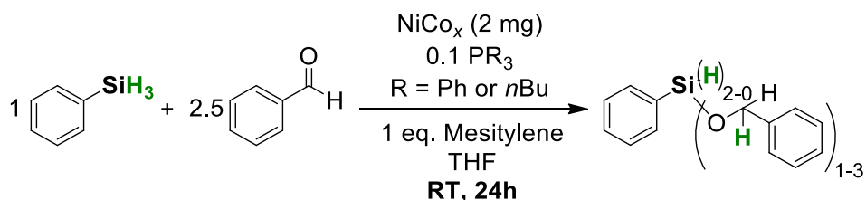
Scheme 1. Catalytic conversion of phenylsilane in the presence of \text{NiCo}_x NPs and a phosphine.
