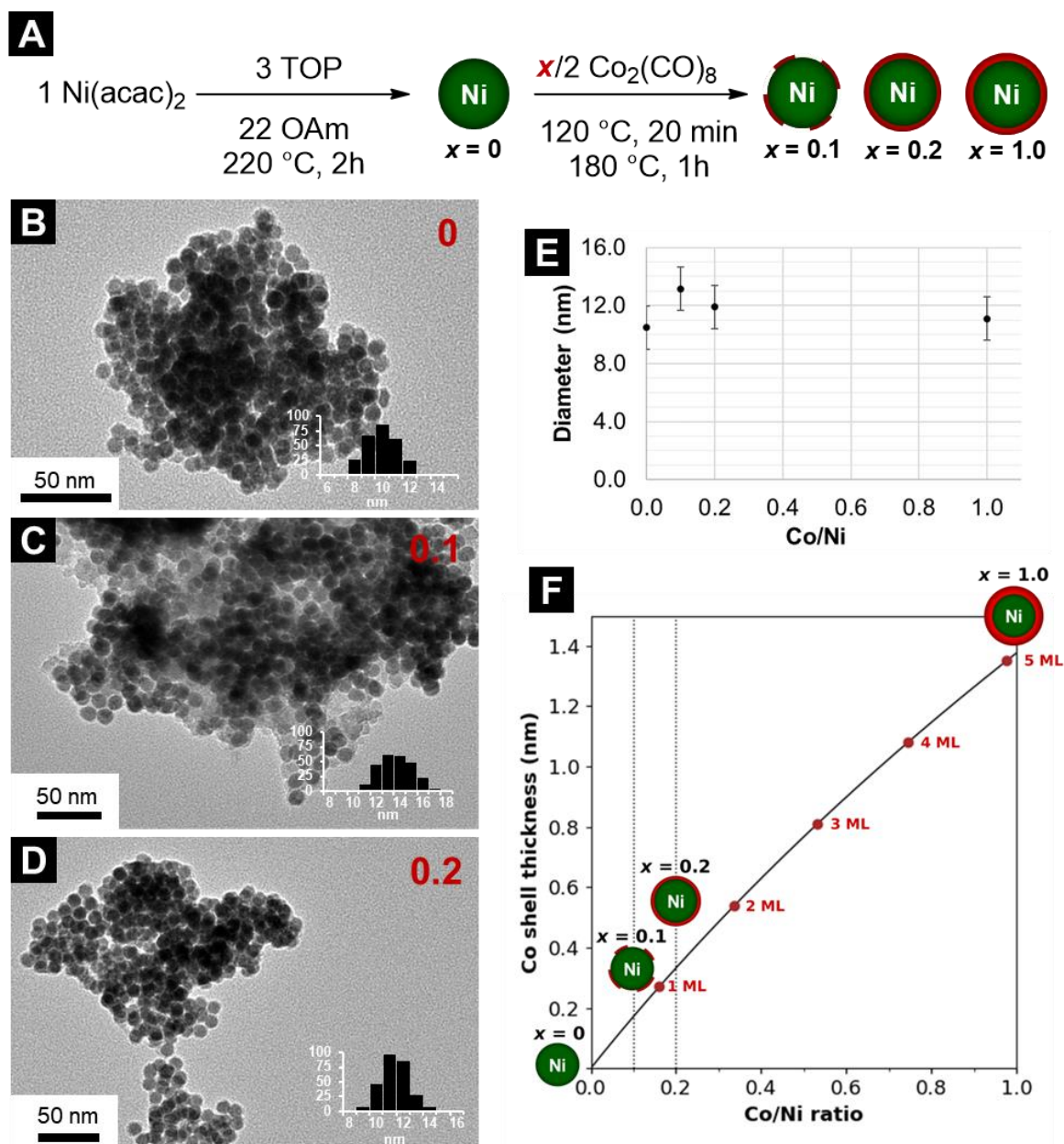
Figure 1. (A) Two-step synthesis of NiCo x nanoparticles. TEM pictures and size distributions for samples with various Co/Ni ratio (B) x = 0 , (C) x = 0.1 , (D) x = 0.2 . (E) Average diameters and (F) geometrical model of the Co shell thickness related to the Co/Ni ratio, where each red dot from left to right shows the formation of successive monolayers (ML).
