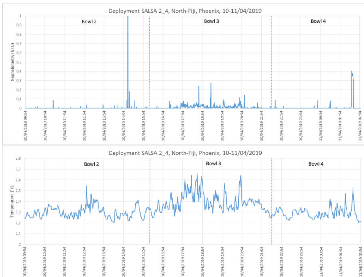
Figure 10: Nephelometry (top) and temperature (bottom) profiles recorded during SALSA2 sampling at Phoenix near communities in active area (Dive 724).
