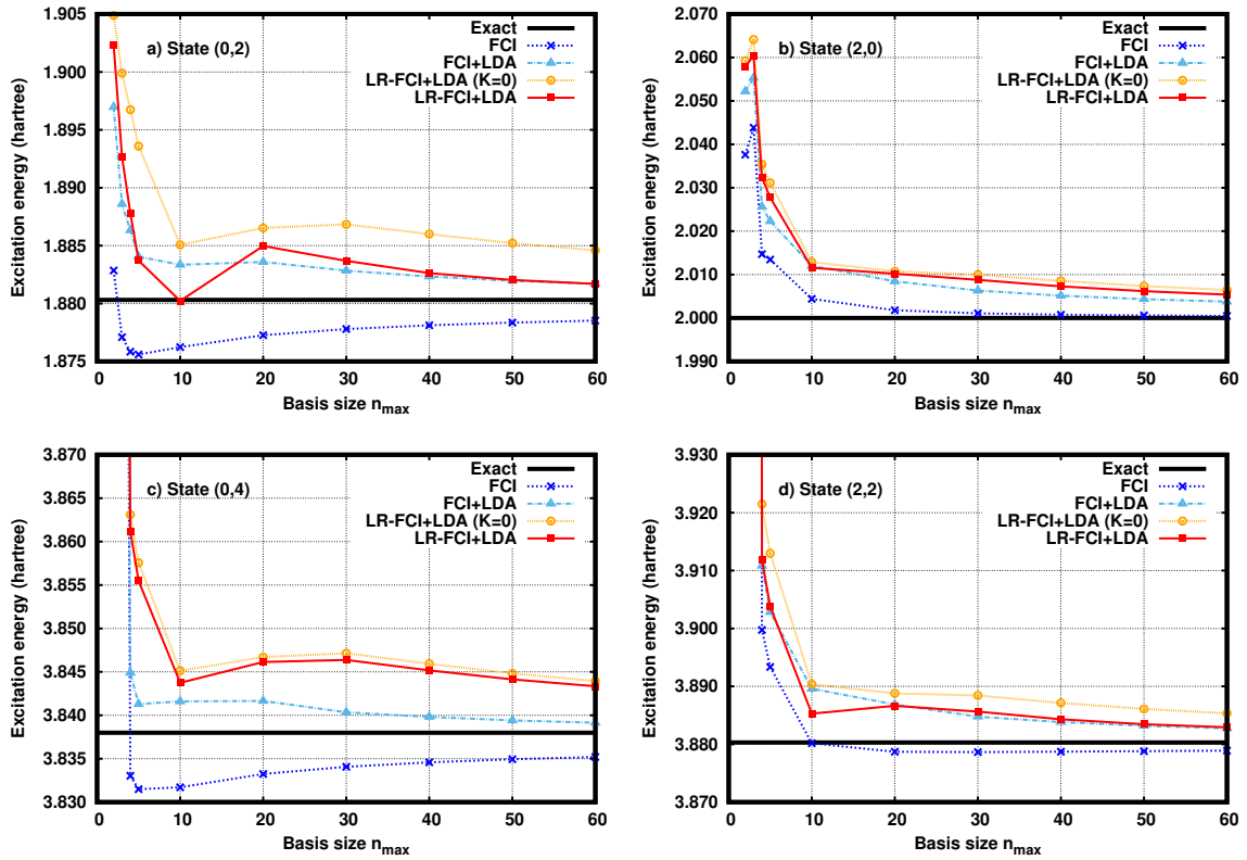
FIG. 2: Excitation energies of the states (0, 2), (2, 0), (0, 4), and (2, 2) of the 1D two-electron Hooke-type atom with \omega_0 = 1 calculated by the standard FCI method and the LR-FCI+LDA basis-set corrected method as a function of the basis size n_{\max} . For comparison, excitation energies obtained with a zero basis-set correction kernel [LR-FCI+LDA (K=0)] and with a non-self-consistent state-specific approach (FCI+LDA) are also shown.
