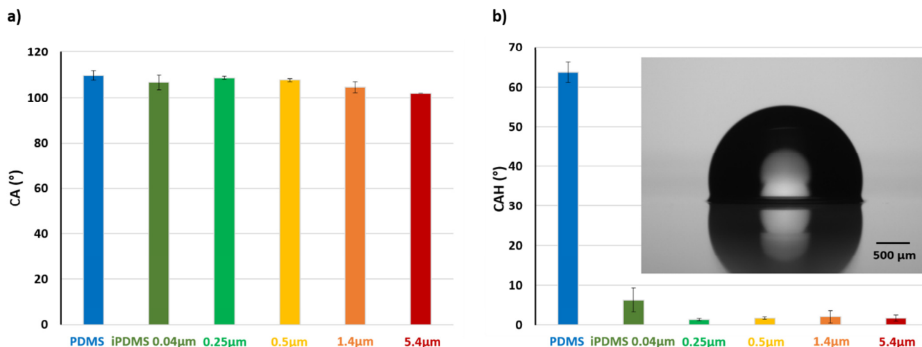
Figure 2: Wetting properties: Static contact angle (CA) and contact angle hysteresis (CAH) of water on PDMS and iPDMS with different oil thickness ranging from 40 nm to 5.4 μm.
