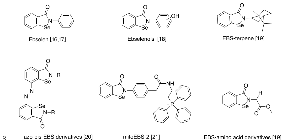
Fig. 1. EBS-related compounds with anticancer activity
