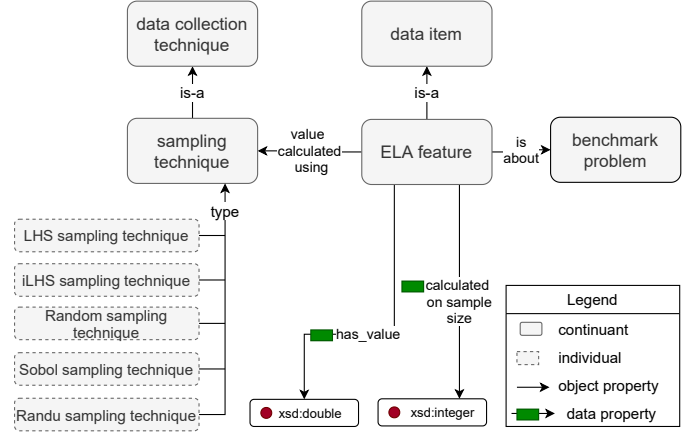
Fig. 3. Representation of ELA features in the OPTION ontology.
