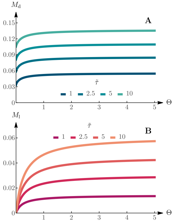
FIG. 1. Steady-state drag coefficient M_d (A) and lift coefficient M_l (B) as a function of the dimensionless inverse compressibility \Theta = (\tilde{\chi}\tilde{\kappa})^{-1} for different values of the relaxation time \tilde{\tau} and for \tilde{\eta}_b = \tilde{\eta}_o = 1 .
