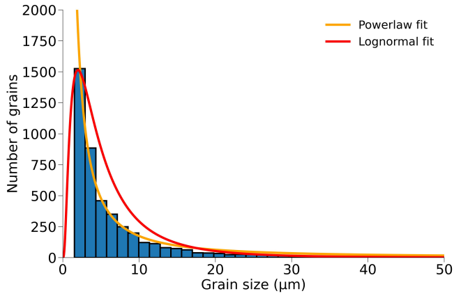
Figure 1. Grain size distribution of olivine. The grain size is the Feret’s diameter computed using SEM images. The red curve is the lognormal distribution fit to the data. The orange line represents the power-law fit to the data.
