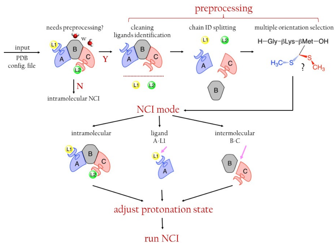
Figure 2: Schematic representation of the workflow of NCIWEB from the input of the PDB structure to the submission of the NCI calculation.
