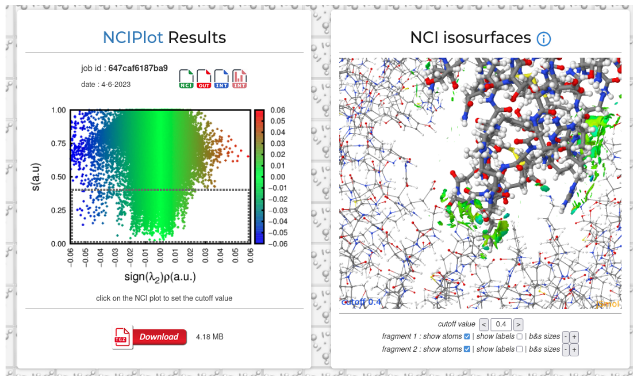
Figure 4: NCIWEB results for intermolecular interaction of ribonuclease inhibitor and ribonuclease A complex (PDB ID: 1DFJ), including the visualization of the resulting 2D NCI plot and of the 3D intermolecular NCI regions at s = 0.4 .
