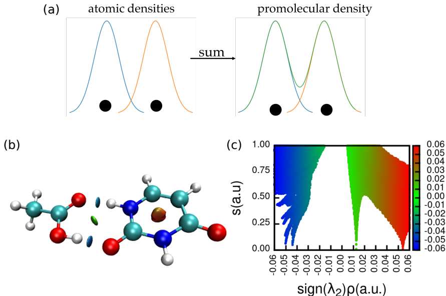
Figure 1: (a) Schematic representation of the promolecular density in one dimension. (b) 3D representation of non-covalent interactions in the AcOH-uracil system and (c) its respective 2D plot. Attractive (blue), van der Waals (green) and repulsive (red) non-covalent interactions are detected.
