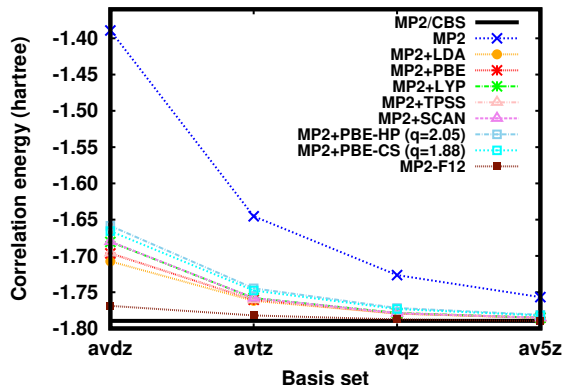
FIG. 1: Basis-set convergence of the ground-state MP2 correlation energy of the tetramethylpentane molecule ( C_9H_{20} ) with different basis-set correction density-functional approximations (evaluated at the HF density) and with MP2-F12 using avnz basis sets.
