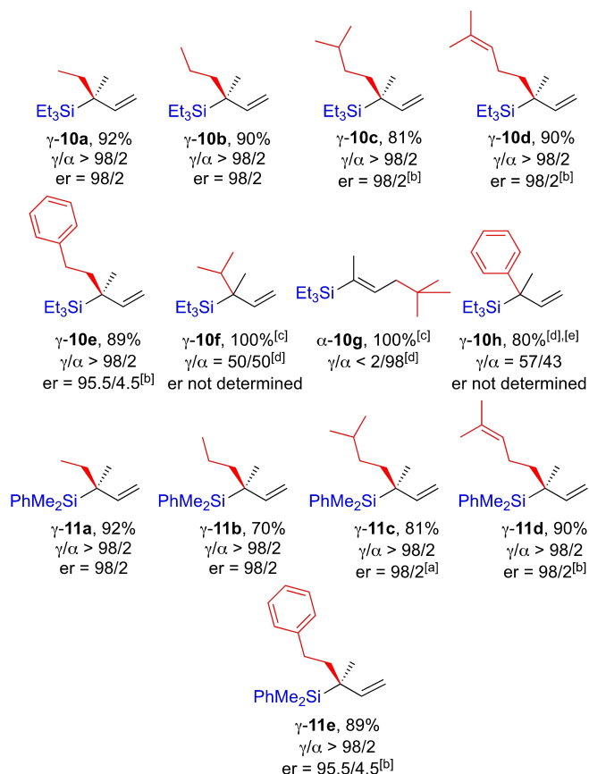
Scheme 3. Transition-metal-free enantioselective synthesis of quaternary \alpha -chiral allylsilanes. \gamma - and \alpha - regioisomers. Isolated yields of inseparable \gamma - and \alpha - regioisomers. Unless otherwise stated. Unless otherwise stated, \gamma/\alpha ratios were determined by ^1\text{H} NMR analysis of crude mixture and er were determined by GC or chiral HPLC analysis. [a] er determined by chiral HPLC analysis of the acryloyl ester after cross-metathesis. [b] er determined by chiral HPLC analysis of the alcohol obtained by hydroboration and subsequent oxidation of the carbon-carbon double bond. [c] Conversion by ^1\text{H} NMR. [d] Side-product detected. [e] 72 h reaction time.
