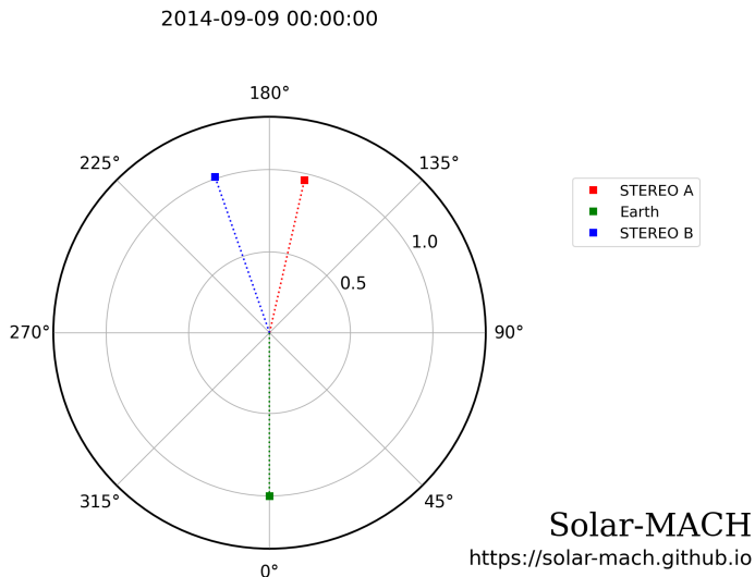
Fig. 2. Position of STEREO-A, STEREO-B, and Earth on September 9, 2014, at 00:00. The grid in black corresponds to the Stonyhurst coordinate systems. This polar plot is generated using the Solar-MACH tool ( https://serpentine-h2020.eu/tools/ ; Gieseler et al. 2022).
