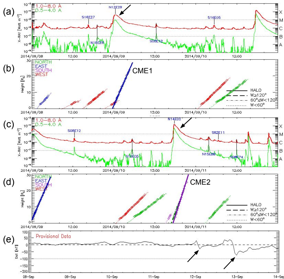
Fig. 1. Overview of the eruption, early evolution in corona, and geomagnetic signatures of CME1 and CME2. Panels (a,b) and panels (c,d) span the time ranges of September 8–10, 2014, and September 9–11, 2014, respectively. (a) M-class flare on late September 8, 2014 (indicated with black arrow), which can be associated with the eruption of CME1. (b) Height-time plot of CME1 shown by the blue height profile starting at \sim 23.30 UT on September 8, 2014. (c) X-class flare on September 10 (indicated with black arrow), which can be associated with the eruption of CME2. (d) Height-time plot of CME2 shown by the purple height profile starting at \sim 17.30 UT on September 9, 2014. The solar source coordinates of the flares are labelled in the GOES X-ray intensity plots in panels (a,c). The colour (line) codes in panels (b,d) define the CME propagation direction (apparent angular width). (e) Disturbance storm index (Dst), a measure of the geomagnetic activity at Earth shows a calm phase followed by a mild disturbance and then a moderate storm in the period 12–14 September, 2014 (disturbances indicated with arrows). Source: CDAW catalogue – https://cdaw.gsfc.nasa.gov/CME_list/daily_plots/sephtx/2014_09/
