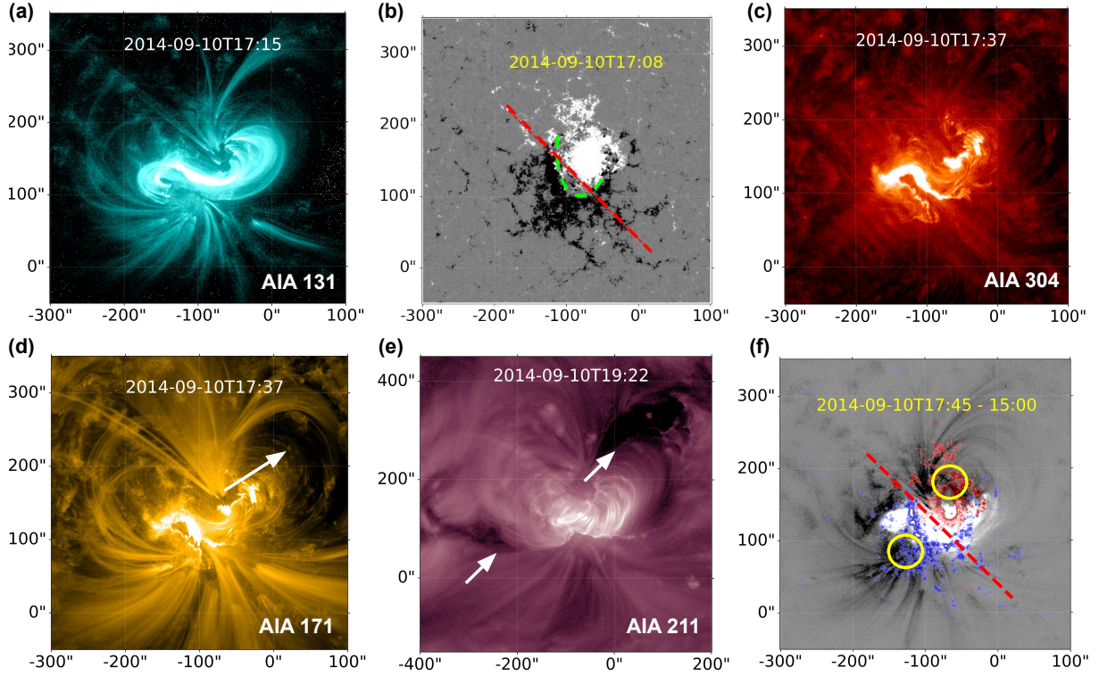
Fig. 6. AR 12158 associated with CME2 eruption in different wavelengths. (a) AIA 131 Å image before CME2 eruption. (b) HMI magnetogram saturated at \pm 200 G overlaid with the approximated PIL drawn with a red dashed line. (c) AIA 304 Å image highlights the inverse J-shaped flare ribbons indicating left-handedness of the flux rope. (d) AIA 171 Å image showing the coronal loops and the eruption direction of CME2 in north-westward direction as per Dudík et al. (2016). (e) AIA 211 Å image showing coronal dimmings marked with white arrows. (f) AIA 131 Å base-difference image overlaid with HMI magnetogram contours saturated at \pm 1000 G coloured blue and red for negative and positive polarity, respectively. The yellow circles demarcate the dimmings located at the footpoints of the FR. The red dashed line is the approximated PIL. The X- and Y-axes correspond to the helio-projective longitude and latitude, respectively.
