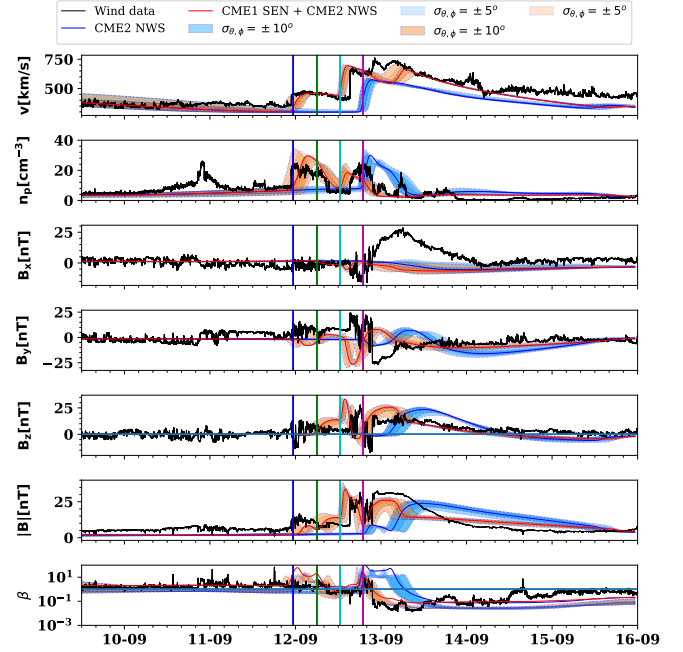
Fig. 12. Results of Run2 (blue; CME2 NWS) and Run4 (red; CME1 SEN + CME2 NWS) are compared. CME1 and CME2 parameters in Run3 and Run2, respectively. Figure description is similar to Fig. 10. S1, the start of ME1, S2, and the start of ME2 are marked with blue, green, cyan, and magenta vertical lines, respectively, in Run4.
