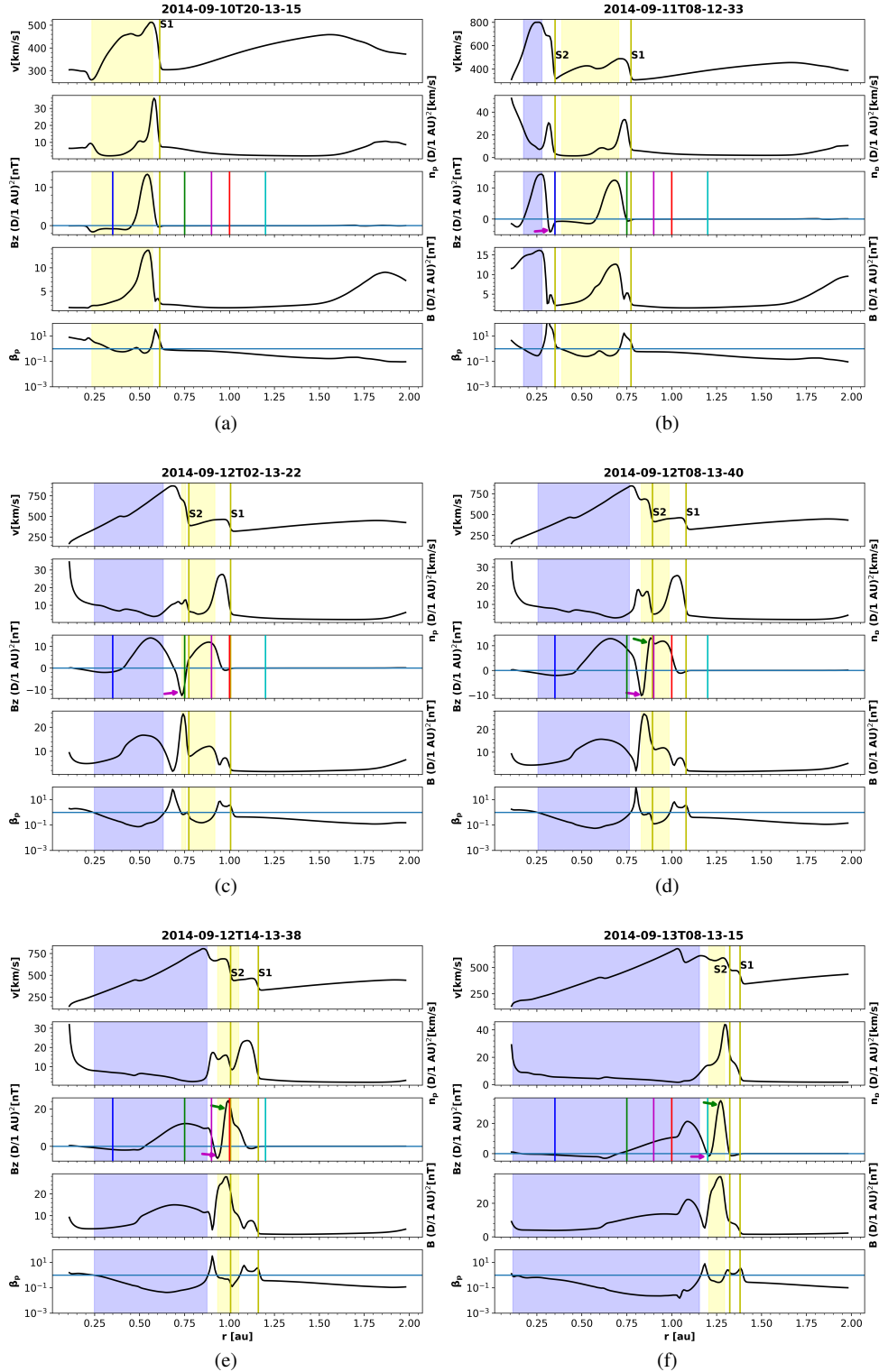
Fig. 13. Radial evolution profile of the CME1 and CME2 along the Sun–Earth line at different times of propagation and interaction extracted from Run4. Top to bottom (in each plot): speed ( v ), proton number density ( n_p ), z -component of magnetic field ( B_z ), total magnetic field ( B ), and proton plasma beta ( \beta_p ). The yellow and blue shaded areas depict the extent of magnetic ejecta of CME1 and CME2, respectively, extracted using the criterion \beta_p < 1 ( \beta_p < 5 in (a)). All physical quantities except the speed are scaled by (D/1 \text{ au})^2 where D is the radial distance from the Sun. The CME shocks (S1 and S2) are marked in yellow lines. The colourful vertical lines in the B_z panel correspond to different radial distances, which help to explain the various phases of Run4 (detailed in Sect. 6.3): (a) Propagation of CME1 alone in the heliosphere; (b) formation of a compressed negative B_z ejecta CE1a (shown with the magenta arrow); (c) further compression of CE1a; (d) development of a compressed positive B_z ejecta, CE1b (shown with a green arrow), ahead of CE1a; (e) further compression of CE1b; and (f) diffusion of CE1a ( \sim 0 nT) upon reaching 1.2 au while CE1b undergoes further enhancement.
