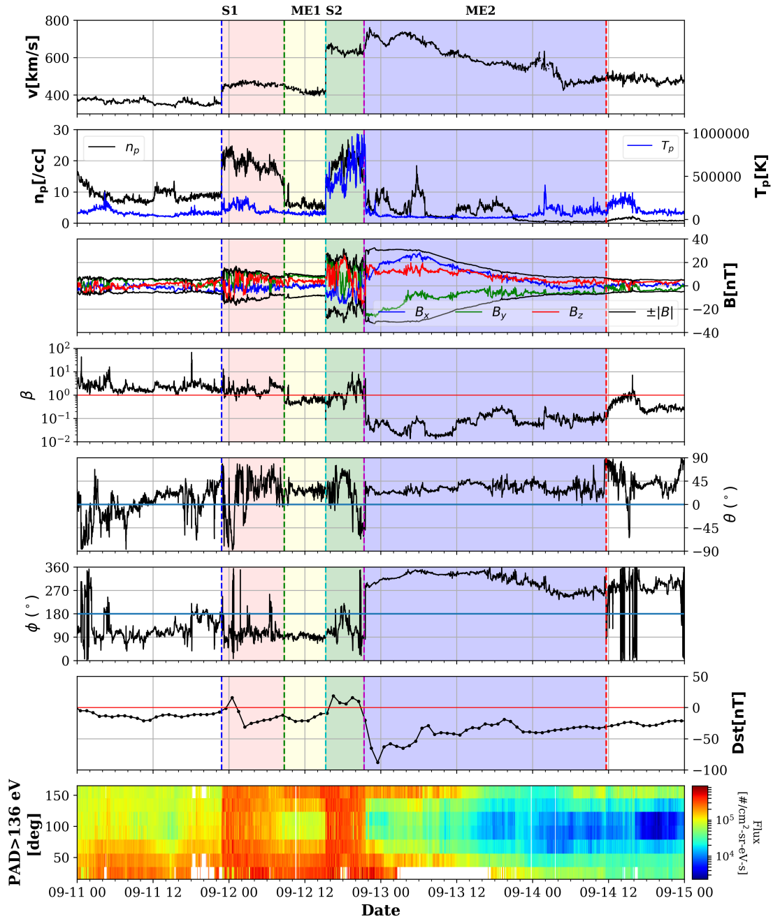
Fig. 4. In situ measurements by the Wind spacecraft during the period of September 11, 2014, and September 15, 2014. The figure shows (top to bottom) speed ( v ); proton temperature ( T_p ) and number density ( n_p ) in the second panel; magnetic field components ( B_x , B_y , B_z ) in the GSE coordinate system capped with the total magnetic field ( \pm|B| ) in the third panel; plasma beta ( \beta ) in the fourth panel; the \theta and \phi components of the magnetic field in GSE angular coordinates in the fifth and sixth panels, respectively; the Dst index in the seventh panel; and the suprathermal pitch angle distribution (with energies >136 eV) in the bottom panel. Vertical dashed lines indicate the shock arrival of CME1 (S1, blue) and the start of the magnetic ejecta passage of CME1 (ME1, green). The shock arrival of CME2 (S2, cyan), the start of the magnetic ejecta passage of CME2 (magenta), and the end of the magnetic ejecta passage (red) are as identified in the Wind ICME catalogue. The shaded red and yellow regions represent the sheath ahead of CME1 and the magnetic ejecta, ME1, respectively. The shaded green and blue regions depict the sheath ahead of the CME2 and the magnetic ejecta, ME2. The magnetic ejecta of CME2 has been identified in the Richardson and Cane catalogue as well.
