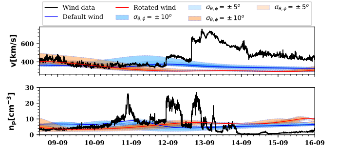
Fig. 9. Background solar wind modelled with the default EUHFORIA coronal model setup using the synoptic magnetogram from GONG on September 8, 2014, at 23:00 (in blue), and the rotated solar wind (in red). The shaded regions provide an error estimate in \pm 5 – 10^\circ in latitude ( \sigma_\theta ) and longitude ( \sigma_\phi ) around Earth. Corresponding WIND observations are plotted in black.
