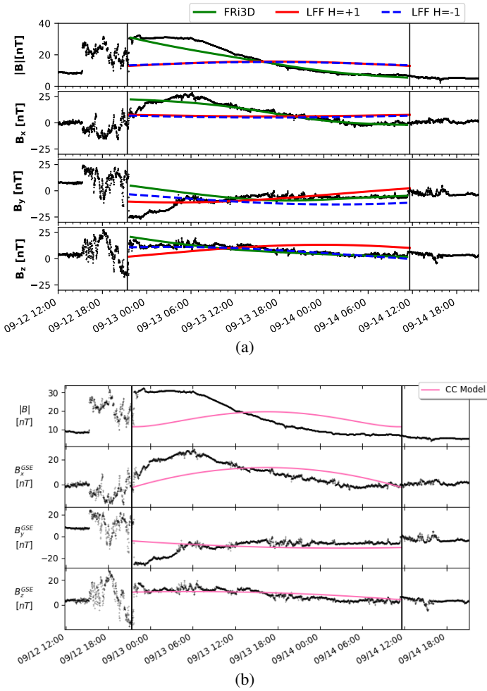
Fig. 7. Fitting of in situ observations of ME2 at 1 au with various models: (a) FRI3D model (green), LFF fit with right-handed chirality (red), and LFF fit with left-handed chirality (blue); (b) CC fit adapted from the WIND ICME catalogue (Nieves-Chinchilla et al. 2018). The vertical lines in black in both plots correspond to the ME2 boundary as per the same catalogue. The fitted parameters of the model are discussed in Sects. 4.1–4.3.
