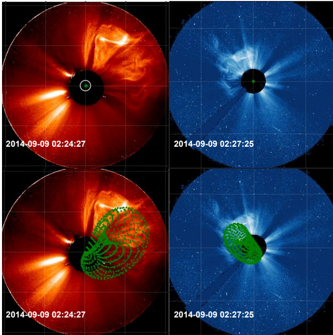
Fig. B.1. Coronagraph images of CME1 development on September 9, 2014, as observed by COR-2 (STEREO-B) and C3 (LASCO) (top). The same images overlaid with the 3D reconstruction using the GCS model (bottom).
