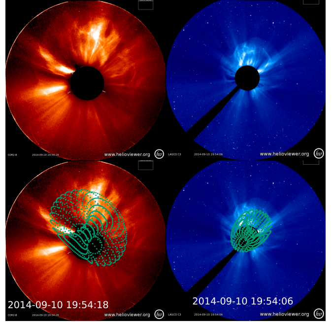
Fig. B.2. Coronagraph images of CME2 development on September 10, 2014, as observed by COR2 (STEREO-B) and C3 (LASCO) (top). The same images overlaid with the 3D reconstruction using the FRi3D model (bottom).
