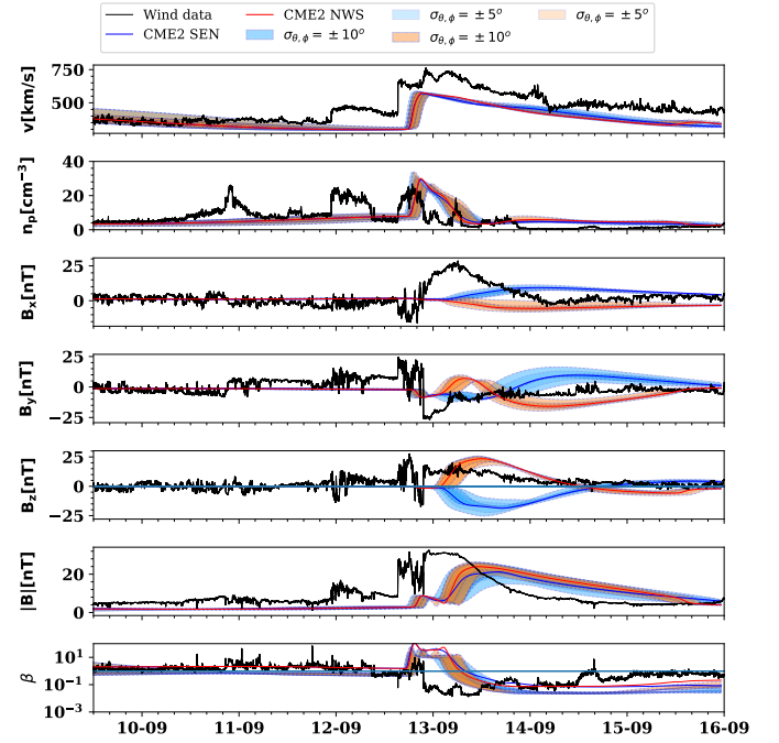
Fig. 10. Time series plot showing a comparison between the simulations with different orientations of CME2 modelled with FRi3D, at Earth: Run1 (blue) is simulated with tilt 0.1 au SEN (deduced based on the orientation close to 1 R_\odot ) and Run2 (red) with tilt 0.1 au NWS (similar to the tilt at 1 au). Both the orientations follow the same geometrical tilt derived from the 3D reconstruction at 0.1 au but with two different axial magnetic field orientations. From top to bottom: Speed ( v ), proton number density ( n_p ), B_x , B_y , B_z , magnetic field strength ( |B| ), and plasma beta ( \beta ). The solid line and the shaded regions show the profile at Earth and in the 5 – 10^\circ latitudinal and longitudinal offset around Earth, respectively.
