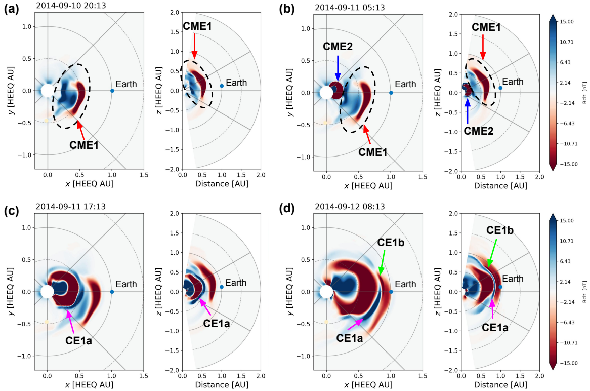
Fig. 14. Evolution of B_z in the heliosphere as simulated in Run4. The co-latitude component in the spherical coordinate system is B_{\text{clt}} , which is equivalent to -B_z on the ecliptic plane. The red and blue spectra of the colour bar correspond to positive and negative B_z , respectively. Each of the panels (a) to (d) shows the view of the equatorial (X–Y) plane and the meridional (X–Z) plane at a particular time, mentioned at the top of each. (a) CME1 in the pre-interaction phase is identified schematically with a dashed ellipse; (b) CME2 is shown evolving behind CME1 in the early stage of interaction; (c) CME2 is seen compressing the interval of the trailing negative B_z component of CME1 to create CE1a (darker blue region) in the sheath ahead of itself; and (d) CE1a is seen to be further compressing the interval of the leading positive B_z component of CME1 to create CE1b (darker red region) during the interaction phase of the event. The animation of this figure can be found online .
