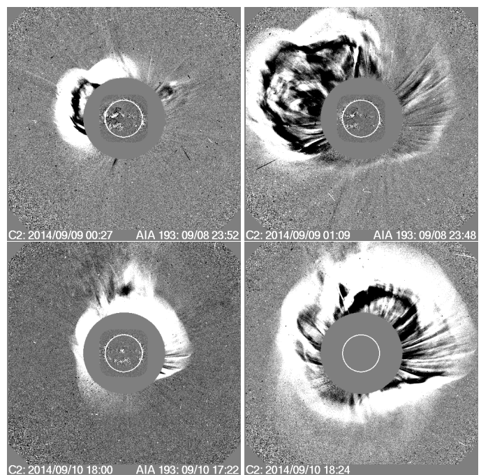
Fig. 3. Running difference images showing the development of CME1 (top row) on early September 9, 2014, and CME2 (bottom row) on September 10, 2014, in the LASCO C2 field of view. Source: https://cdaw.gsfc.nasa.gov/CME_list/
