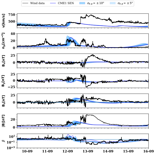
Fig. 11. Results of Run3 where CME1 is modelled with the spheromak model. The figure description is similar to that of Fig. 10.
