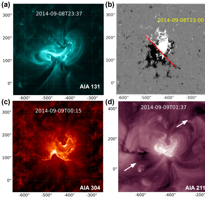
Fig. 5. AR 12158 associated with CME1 eruption in different wavelengths. (a) AIA 131 Å image highlighting the evolved sigmoid and the hooks corresponding to flux rope footpoints during the early phase of the flare. (b) HMI magnetogram saturated at \pm 200 G overlaid with the approximated PIL orientation (i.e. the part of the extended PIL that most likely erupted as CME1), before the start of the flare. (c) AIA 304 Å image showing the inverse J-shaped flare ribbons after the eruption, which suggest the eruption of a left-handed flux rope. (d) AIA 211 Å image showing the post-flare coronal dimmings (marked with white arrows). The X- and Y-axes correspond to the helio-projective longitude and latitude, respectively.
