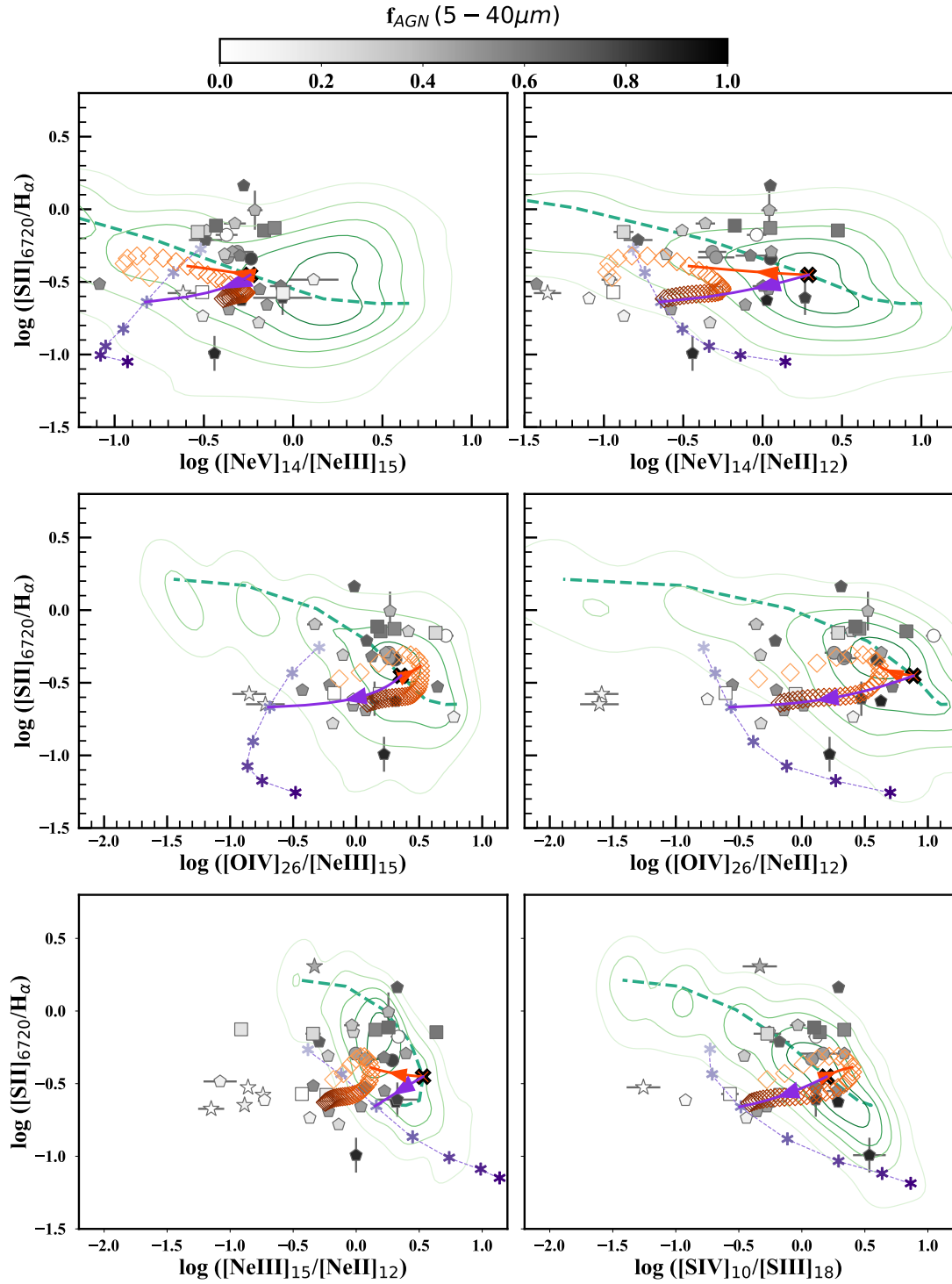
Fig. A.5. Examples of [S II] versus mid-IR ratio diagrams. Symbols and colors of the observations and models are the same as in Fig. 5.
