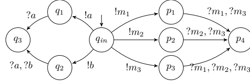
■ Figure 13 Wait-only protocol \mathcal{P}_2 .
