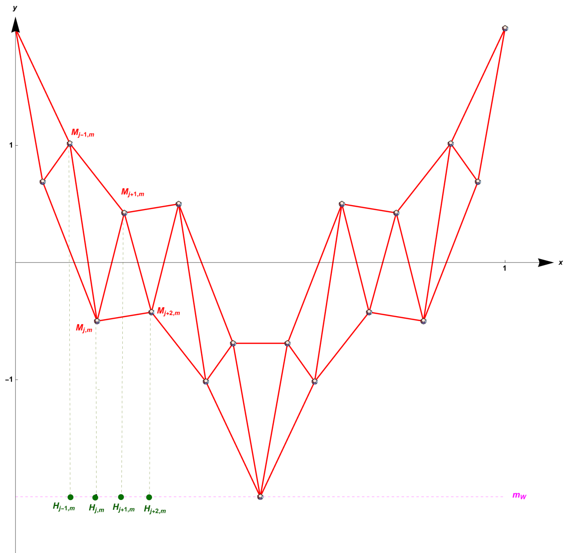
Figure 10. The orthogonal projections H_{j,m} of the vertices M_{j,m} , for 0 \leq j \leq \#V_m - 1 , onto the horizontal line y = m_{\mathcal{V}} , where m_{\mathcal{V}} is introduced in Notation 29, on page 17.
