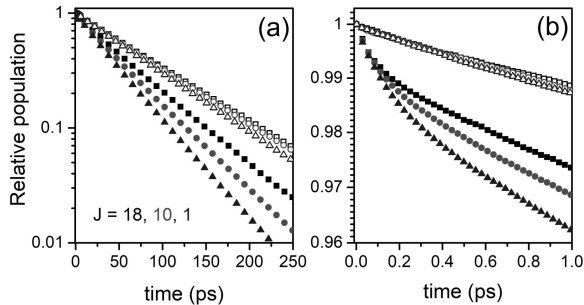
FIG. 3. Computed (see text) populations, normalized to unity at t = 0 , for CO diluted in N_2 (full symbols) and He (open symbols) at 296 K and 101.3 kPa (1 atm) for three rotational quantum numbers J shown over extended (a) and reduced (b) time scales.
