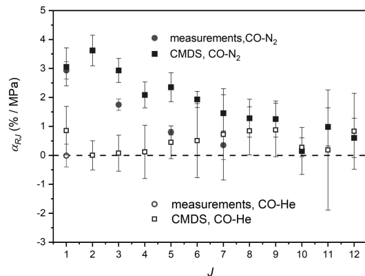
FIG. 2. Intensity-correction slopes obtained from measured (circles) and computed (squares) spectra versus the lower-state rotational quantum number J for RJ lines for CO-N _2 (full symbols) and CO-He (open symbols).
