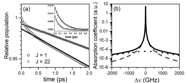
FIG. 4. (a) Exponential decay functions (lines) obtained from fits, at long time delays, of the relative populations (symbols) computed for J=1 and J=22 at 296 K and 101.3 kPa. The insert shows the differences between the latter and the former as well as their exponential fits. (b) The line spectrum for J=1 (full line) calculated as the Fourier-Laplace transform of the relative population \rho_{J=1}(t) . The dashed and dotted lines represent the narrow and broad contributions associated respectively with the long- and short-time exponential decays of the populations.
