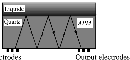
Figure 5. Cross section of a typical APM transducer showing the substrate, the interdigitized electrodes and the fluid sample.
