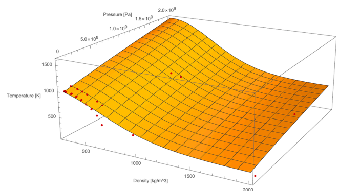
Fig. 1. IAPWS data on the surface plot of \rho(p, T) .
