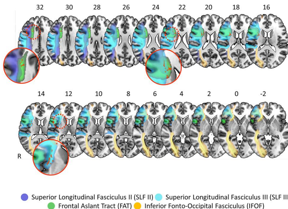
Figure 3 Neuroanatomical analysis. (A) The results of the VLSM analysis using the PCA factor values of the common component (i.e. PCA Component I) as predictive values. The results show two significant lesion clusters (red, with a total volume of 325 voxels). The first and larger cluster (top row) is located within the second branch of the SLF (SLF II, dark blue), the third branch of the SLF (SLF III, light blue) and the FAT (green). The second and smaller cluster (bottom row) is located within the SLF III, the anterior part of the putamen and the IFOF (yellow). Patients with right-hemispheric stroke presenting with a lesion within these clusters were significantly more likely to show an impairment in overall cognitive performance in all three considered cognitive domains, as reflected by the lower factor values in the common component (PCA Component I). (B) The results of the disconnectome map analysis for a ROI including all four white matter tracts identified as affected by the previous VLMS analysis, i.e. the SLF II, the SLF III, the FAT and the IFOF. Patients with right-hemispheric stroke presenting with a lesion within these clusters were significantly more likely to show an impairment in overall cognitive performance in all three considered cognitive domains, as reflected by the lower factor values in the common component. For both panels, lesion voxels that were a significant predictor for the common component factor values are depicted in red (significance level P < 0.05 , based on the Brunner–Munzel test, false discovery rate-corrected, 4000 permutations). Lesion clusters and white matter tracts are displayed on the MNI152 template in MNI space, as available in MRICroGL ( https://www.nitrc.org/projects/mricrogl/ ). The axial slices are oriented according to the neurological convention. The position of each slice in MNI space is indicated by numbers at the top of the respective slices. White matter tracts are depicted according to published probabilistic diffusion tensor imaging atlases 2,59 (the probability of voxels belonging to the SLF II (in dark blue), SLF III (in light blue), the FAT (in green) and the IFOF (in yellow) was set at \geq 50\% ).
