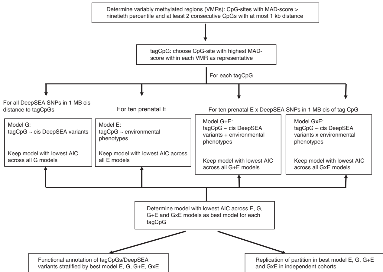
Fig. 1 Flow diagram of VMR analysis
