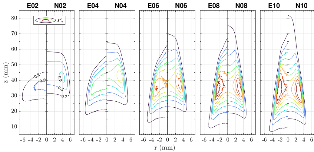
Figure 9: Evolution with the pressure of P_\lambda contours for experimental (E02-E10) and numerical (N02-N10) flames.
