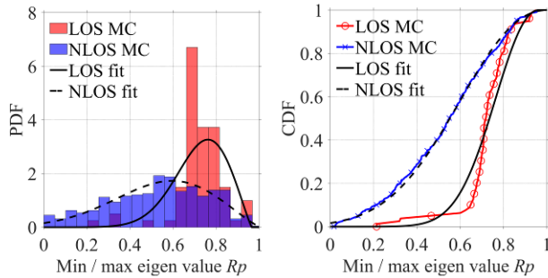
Fig. 14. PDF and CDF of measured covariance eigenvalue ratios R_p .
