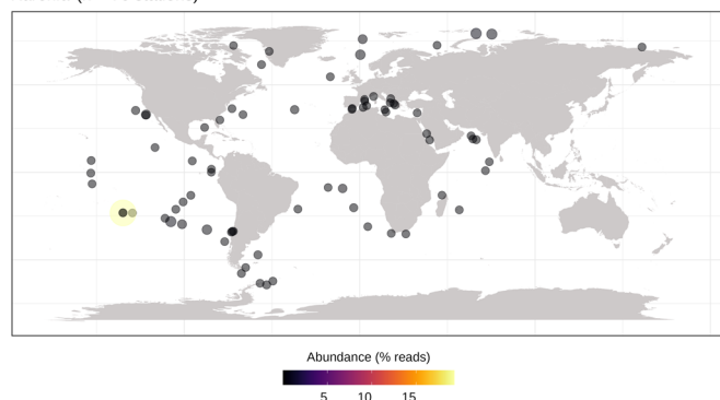
Karlodinium (n = 124 stations)
