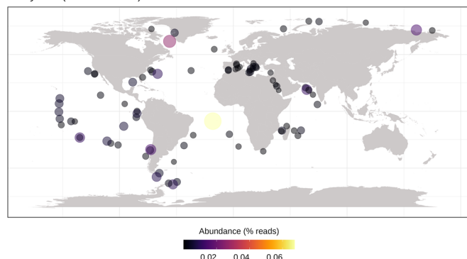
Takayama (n = 84 stations)
