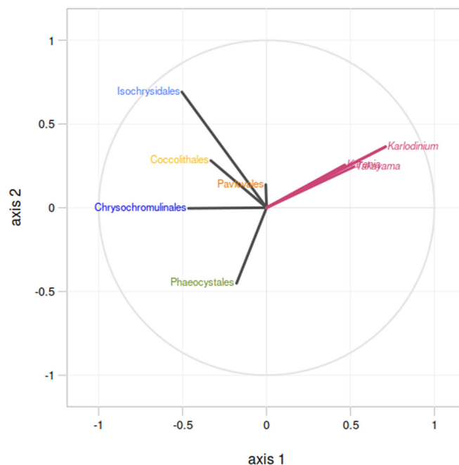
Figure 7. Non-coincidence of karenianaceae and haptophytes in global meta-genome datasets.
