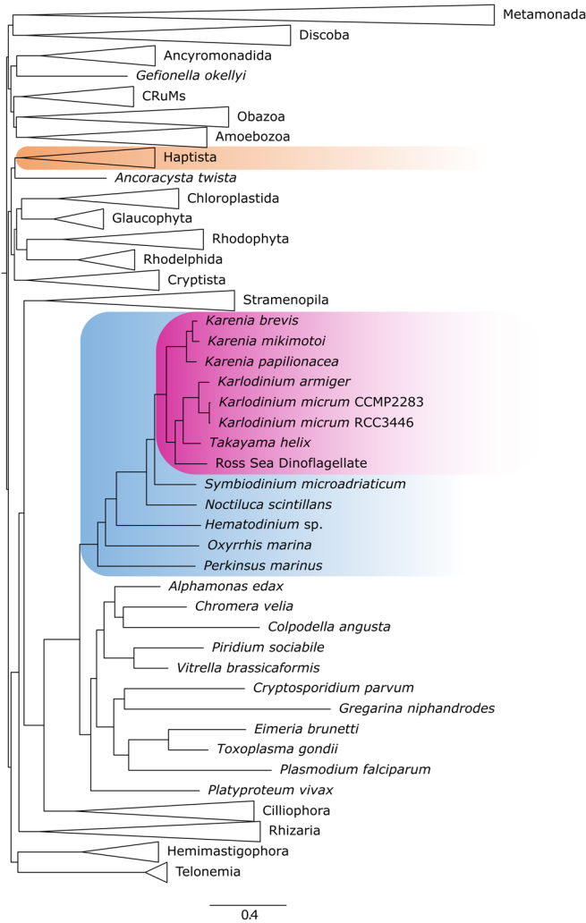
Figure EV1. The eight kareniaceans in the pan-eukaryotic phylogenetic context as reconstructed by IQ-TREE based on a matrix of 241 genes prepared using PhyloFisher toolkit. The inner relationships between the studied kareniaceans are resolved with maximum support and confirm the results of previous phylogenetic analyses based on ribosomal subunits (Takahashi et al, 2019; Ok et al, 2021).
