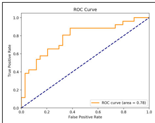
Figure 7. AUC of our ANN-models using EHRs and syn-EHRs.
