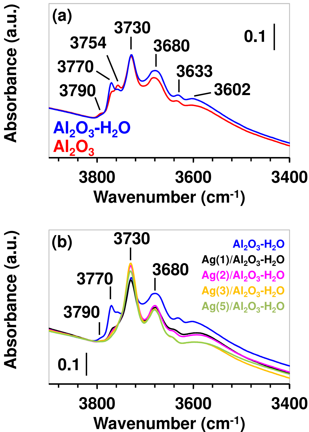
Figure S4. Absorbance FTIR spectra normalized on a 10 mg/cm 2 basis of (a) \text{Al}_2\text{O}_3 and \text{Al}_2\text{O}_3\text{-H}_2\text{O} and (b) \text{Ag}(x)/\text{Al}_2\text{O}_3\text{-H}_2\text{O} samples.
