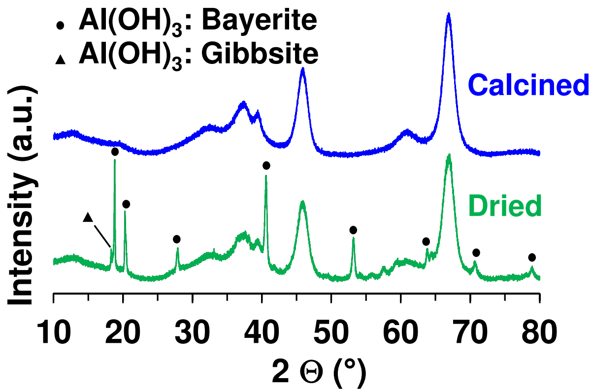
Figure S2. XRD patterns of Al 2 O 3 -H 2 O (treated in water at 80 °C for 66 h) after vacuum drying at RT (green) and calcination at 600 °C for 4 h (blue). \gamma -Al 2 O 3 (JCPDS 79-1558), Bayerite (● JCPDS 20-11) and Gibbsite (▲ JCPDS 33-18).
