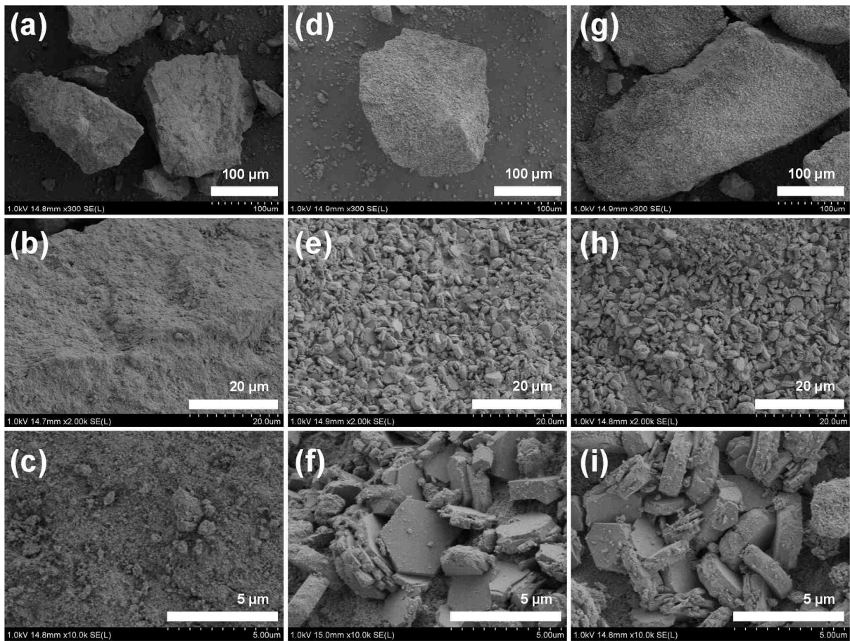
Figure S3. SEM-FEG images at various magnifications of (a-c) the pristine \text{Al}_2\text{O}_3 support ( \text{Al}_2\text{O}_3 ), (d-f) the dried warm-water-pretreated \text{Al}_2\text{O}_3 support and (g-i) the calcined warm-water-pretreated \text{Al}_2\text{O}_3 support ( \text{Al}_2\text{O}_3\text{-H}_2\text{O} ).
