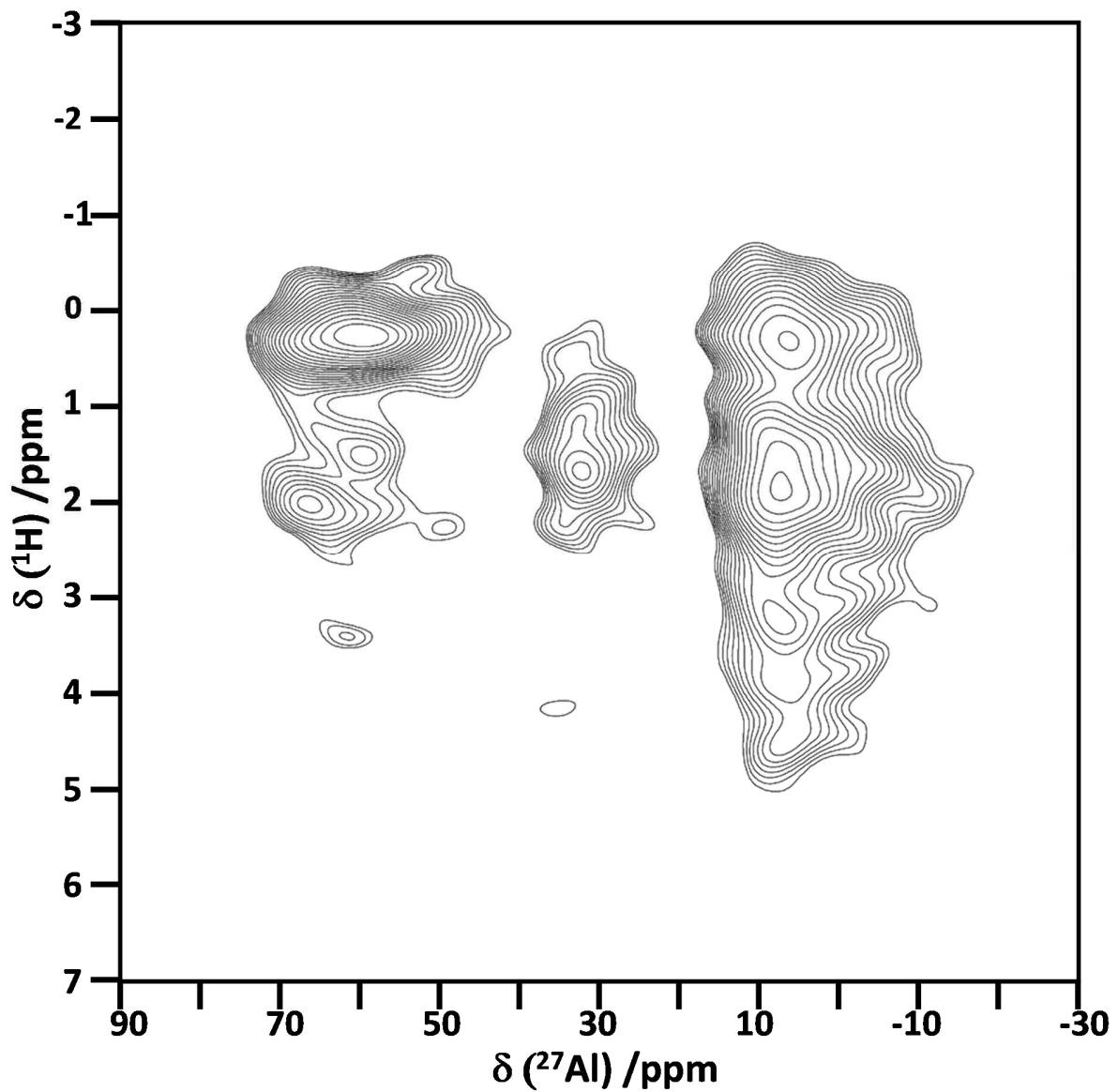
Figure S15. ^1\text{H} - ^{27}\text{Al} D-HMQC MAS NMR spectrum of Ag(1)/Al 2 O 3 .
