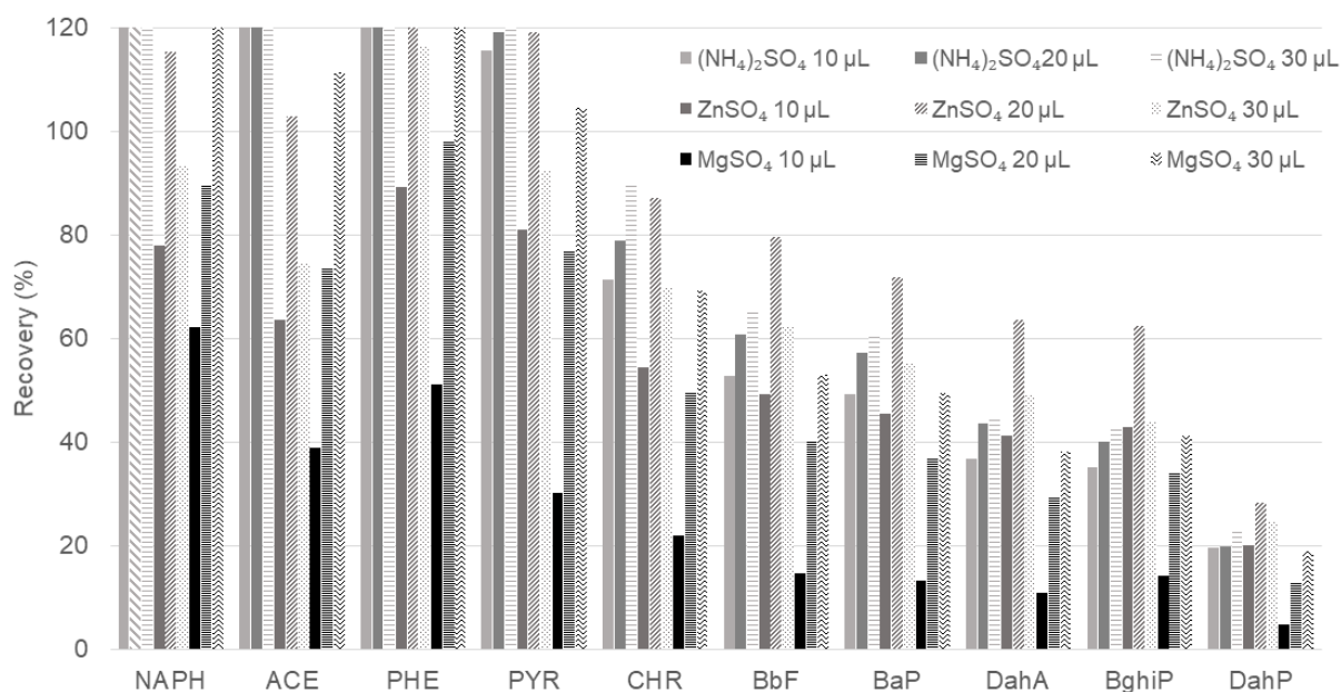
Figure 4 Effect of salt addition in human serum (100 \mu\text{L} ) during the precipitation step with ACN on the extraction recoveries of the 10 representative PAHs ( n=1 ). Extraction conditions: sample spiked at 4.5 \mu\text{g/L} (50 \mu\text{g/L} , 10 \mu\text{L} in ACN); protein precipitation with ACN (100 \mu\text{L} ) + saturated solution of \text{MgSO}_4 , \text{ZnSO}_4 or (\text{NH}_4)_2\text{SO}_4 (10, 20 or 30 \mu\text{L} ); centrifugation (4500 rpm, 30 min, 4°C); supernatant sample (150 \mu\text{L} ) diluted to 1 mL with NaCl 0.5%; extraction solvent/dispersible solvent : 1-dodecanol/MeOH (1/3, 40 \mu\text{L} ); syringe filter (PTFE-HL, diameter: 4 mm, porosity: 0.2 \mu\text{m} ). The figure is truncated from 120%. Other DMLLE-SFO conditions: see Fig. 1.
