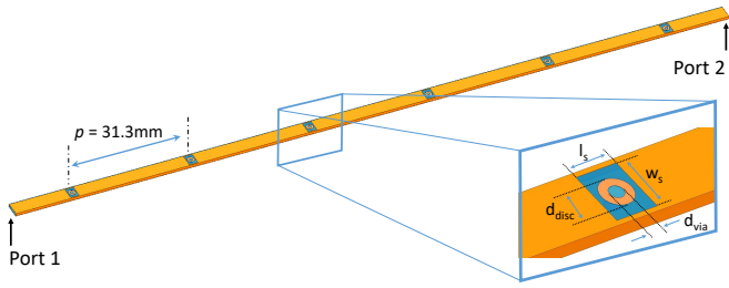
Fig. 1: 6-cells LWA geometry with overall length of 18.78 cm, waveguide width of 3.5 mm, and height of 0.762 mm. Dimensions of rectangular slots with via hole are: l_s = 3 mm, w_s = 2.3 mm, d_{via} = 0.8 mm, and d_{disc} = 1.7 mm. The waveguide is filled with dielectric ( \epsilon_r = 2.94 and \tan \delta = 0.0012 ).
