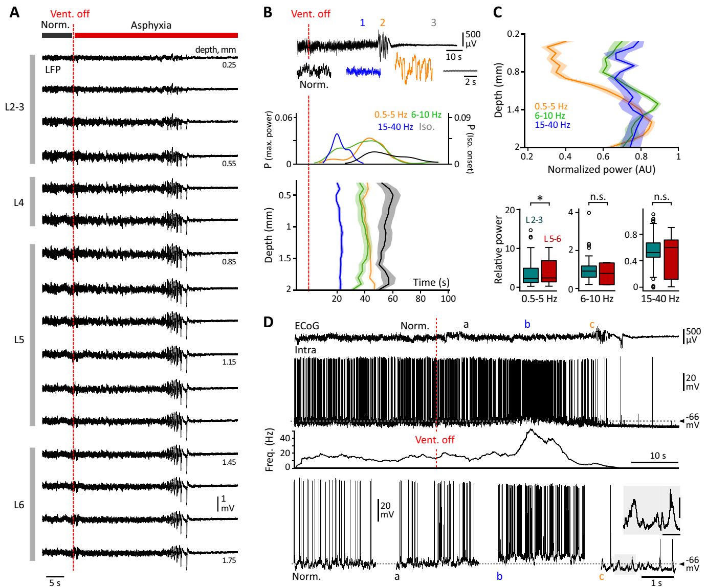
Fig. 2. Anoxia-induced changes in S1 spontaneous activity across layers. (A) LFP activities recorded at different depths of a cortical S1 column with a 32-channel silicone probe (100 \mu\text{m} vertical separation distance between two electrodes), before (Normoxia, Norm.) and after asphyxia induction (Vent. off). Cortical layers (L) are indicated at left. Here, and in the following figures, the recording depth is indicated below the corresponding LFP channel. (B) Representative LFP recording in L5 (top) temporally aligned with the probability densities (P) of maximum power timings for the color-coded frequency bands and of the isoelectric state onset times (grey line) (middle graph). The bottom graph shows, for each frequency band, the mean ( \pm SEM) latency of the maximum powers as a function of cortical depth ( n = 27 protocols). The short recordings in color correspond to expanded views of the normoxic period (Norm.) and of the epochs indicated by numbers above the continuous record. The dashed vertical red line indicates Vent. off. (C) Average ( \pm SEM) distribution of maximal power (normalized to their values during the anoxic period) for each frequency band, as a function of cortical depth. The boxplots compare the power of the different frequency bands in L2-3 and L5-6, relative to their corresponding baseline values. (D) Intracellular activity changes over the anoxic period. Top traces: simultaneous recordings of S1 ECoG and intracellular activity of a L5 pyramidal neuron (Intra), before and after Vent. Off. The horizontal dashed line indicates the mean control V_m ( -66 mV). The graph below shows the corresponding instantaneous firing rate as a function of time. Lower traces are expanded views of intracellular activity recorded during the periods indicated by letters above the ECoG. Norm. corresponds to the normoxic period before Vent. Off and a, b, c corresponds to the early anoxic, high-frequency and low-frequency periods, respectively. In c, spikes are truncated and the inset is a zoom in the slow V_m fluctuations. Calibrations: 6 mV, 200 ms. ns: non-significant; *: P < 0.05 . (For interpretation of the references to color in this figure legend, the reader is referred to the web version of this article.)
