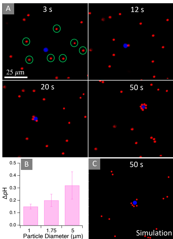
Figure 5: Interparticle potential mediates capture of smaller particles. (A) Sequence of images for 5 μm (blue) surrounded by 2 μm (red) CB-PS particles at the levitated layer under 5 V pp and 100 Hz. A large particle behaves as a beacon for smaller particles, indicated by green circles. (B) Size dependence of ΔpH. Error bars in Panel B represent the standard deviation of values from ten frames and ten different particles, for a total of 100 points. (C) Characteristic result of a Brownian dynamics simulation with interparticle potentials fitted from experimental data and initial configurations from (A, 3s). The simulation domain is a square, with sides equal to 115 μm.
