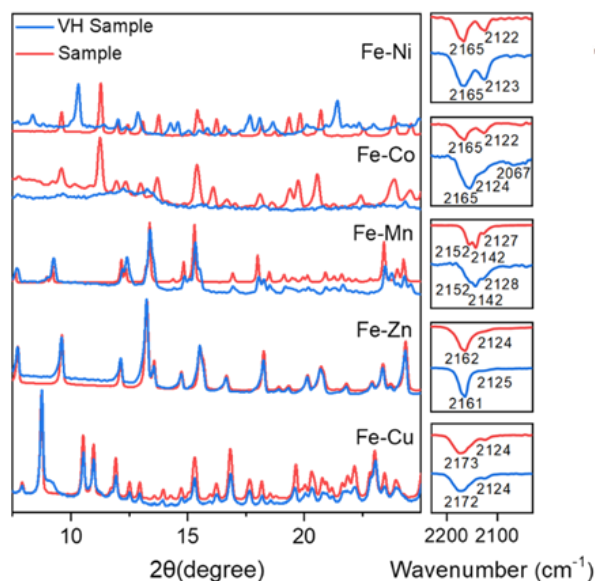
Fig. 3. Powder X-ray diffraction patterns and partial IR spectra of compounds before and after vacuum heating (noted as VH) at 100 °C.
