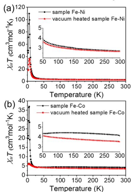
Fig. 4. Thermal dependence of the \chi_M T product of Fe-Ni and Fe-Co in the temperature range 1.9-300 K.
