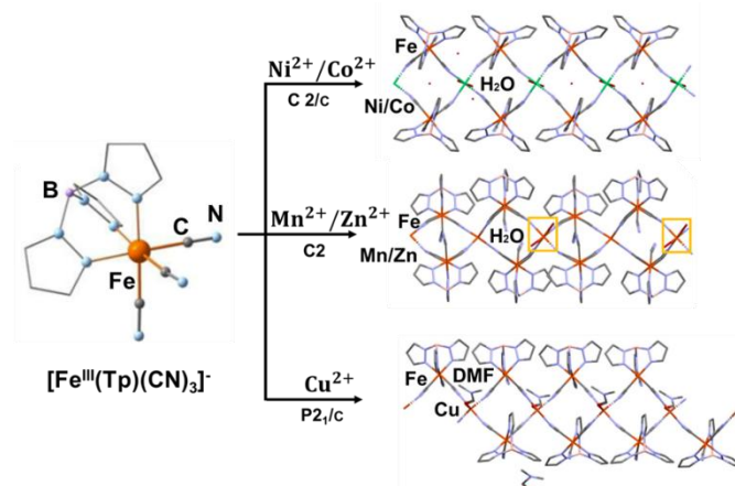
Scheme 1. Schematic illustration for the synthesis of the chain compounds. The draws on the right are perspective views of the (\text{Fe}_2\text{M})_n chain crystal structures.
