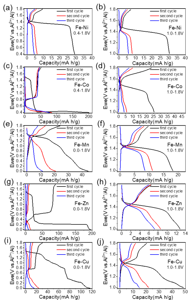
Fig. 5 Galvanostatic discharge-charge profiles of the compounds in the voltage range of 0–1.8V/0.4–1.8V and 1.0–1.8V.
