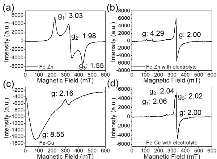
Fig. 8. EPR spectrum of samples (Fe-Zn and Fe-Cu) and sample-electrolyte mixtures at 4 K.
