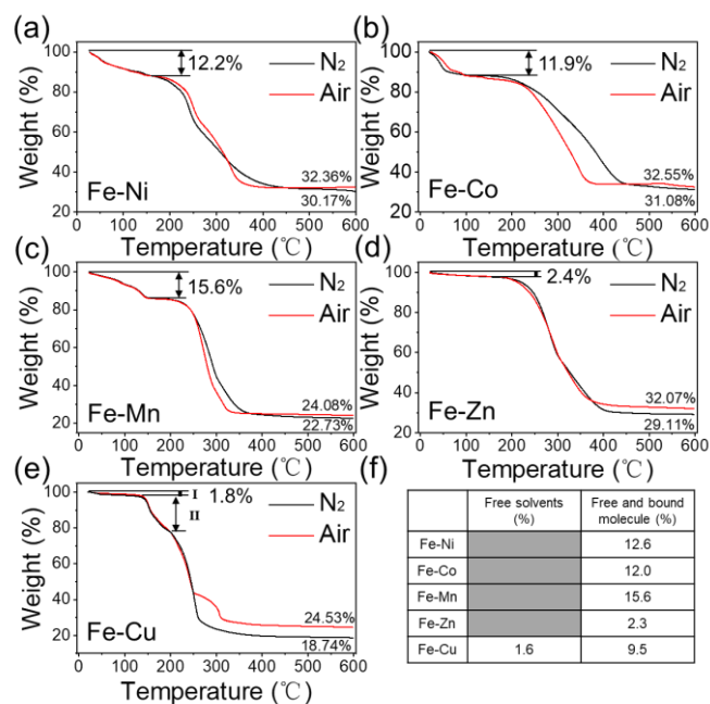
Fig. 2. (a-e) Thermogravimetric analysis of the compounds in nitrogen and air atmosphere; (f) Calculated percentage of solvent to the total weight of the molecule.
