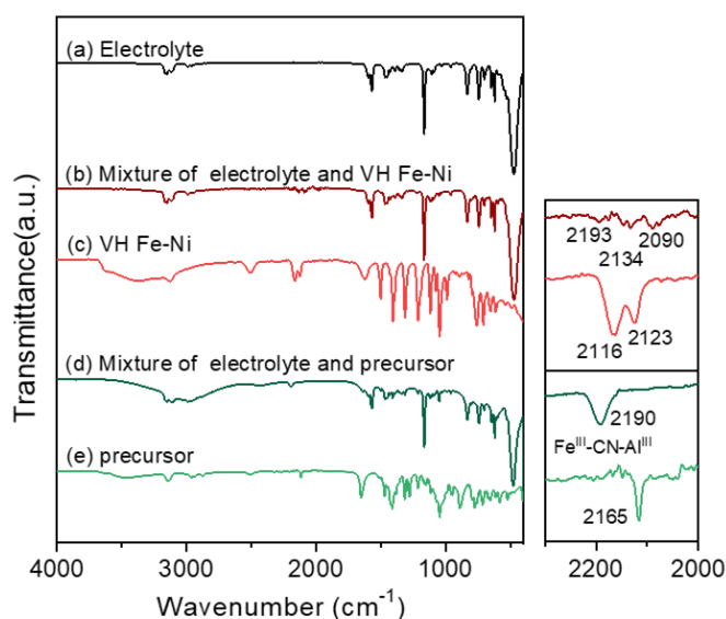
Fig. 9. Infrared spectra of pure electrolyte, sample after vacuum heating (noted as VH) at 100 °C and mixture of electrolyte and samples after vacuum heating: (a) electrolyte; (b,c) Fe-Ni; (d,e) (\text{NBu}_4)[\text{Fe}(\text{Tp})(\text{CN})_3] precursor.
