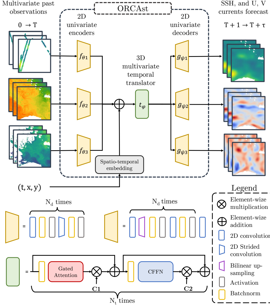
FIG. 4. Overview of ORCAst. Our models inputs temporal sequences of multivariate satellite observations (here SSH, SST, CHL) from t = 0 to t = T . Each variable is inputted to a different spatial encoder, which extracts information from each timestep separately. A spatio-temporal positional embedding is applied to inform the network of geographical coordinates and seasonal information. A spatio-temporal translator t_\varphi is used to produce the forecast encodings. Finally, each timestep is decoded independently with three univariate decoders g_\psi , forecasting SSH, U and V components separately.
