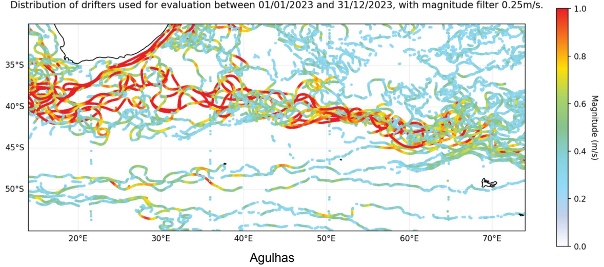
Fig. 2. In situ observations of currents from drifters in three key regions in 2023, used for evaluation.
