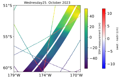
(b) KaRIn-nadir crossings south-east of New-Zealand
