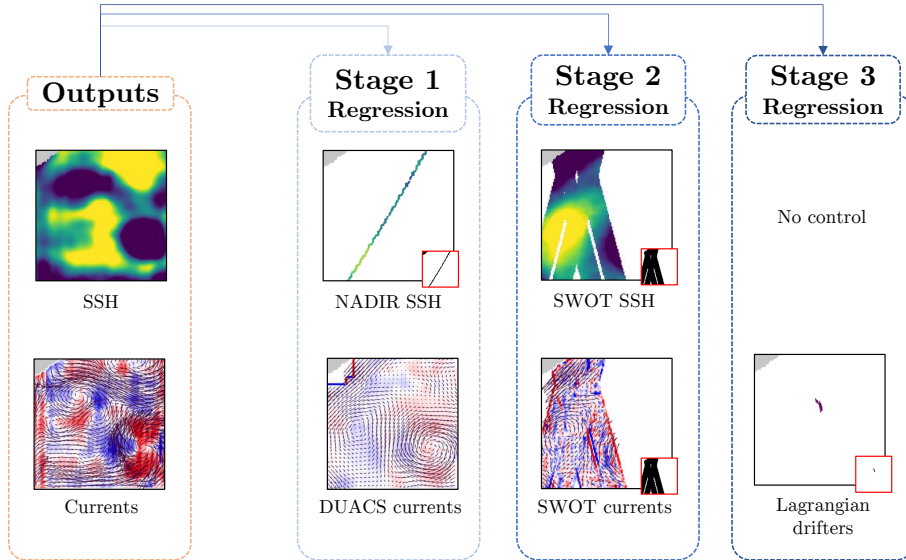
FIG. 5. ORCAst training stages. From left to right, we first show an output example of SSH and U and V components of ocean surface currents, represented as a vector field with colours denoting vorticity. Stage 1 shows nadir and DUACS regression targets, where the small red box illustrates the mask of pixels taken into account when computing the loss. Stage 2 shows SWOT regression targets, with associated masks on the loss function in the small red box. Stage 3 shows drifter regression target, with masks on the loss function in the small red box. Note that in Stage 3 we freeze the SSH decoder and train the model to learn only U and V .
