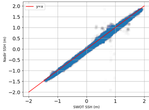
(a) KaRIn vs nadir SSH at overlapping measurements (on the same day at the same location)
