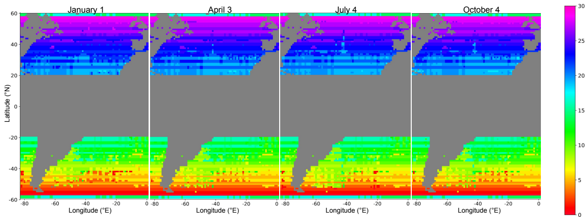
FIG. A3. Clustering of positional embeddings for longitudes 80^{\circ}\text{W} to 0^{\circ}\text{E} at 4 different seasons using k -means, where k = 30 . Each colour represents a cluster learned by our model. We reorder the numbering and colours of the groups for clearer visualisation purposes. Land areas and the equator are in grey.
