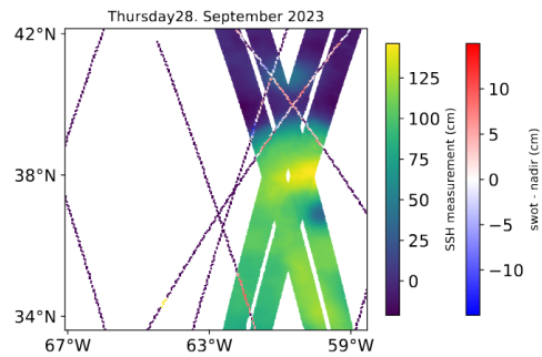
(d) KaRIn-nadir crossings near the Gulf Stream
