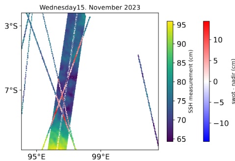
(c) KaRIn-nadir crossings south-west of Singapore
