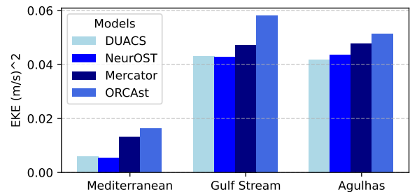
FIG. D1. Eddy Kinetic Energy (EKE) for our three zones of interest.
