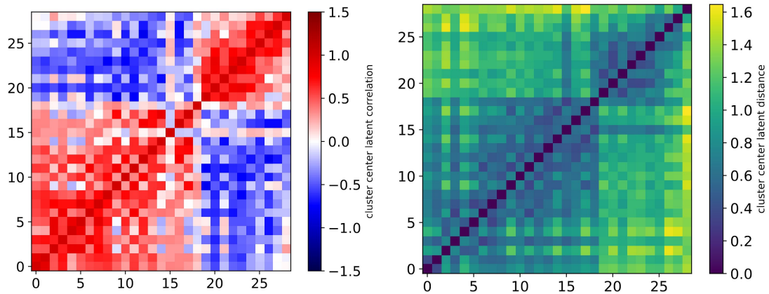
FIG. A2. The correlation (left) and the distance (right) between clusters of our positional embedding, chosen using the k -means method with k = 30 . Geographic zones corresponding to cluster numbers are shown in Figure A1. Southern Hemisphere clusters are numbered 0-18 and Northern Hemisphere clusters are numbered 19-29.
