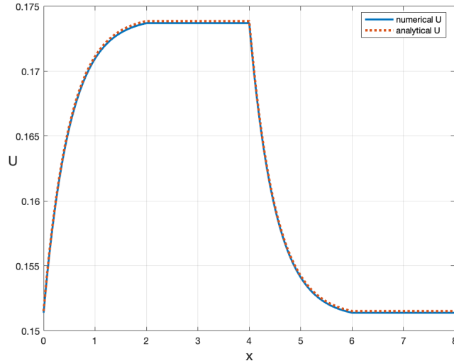
Figure 8: Comparison between the reference solution (in red) and the converged numerical solution (in blue) for the velocity for a laminar flow at small velocities through a thermosyphon with as a number of nodes N_x = 100000 , final time T = 10s , length L = 2m , imposed temperatures at the walls T_c = 300.15K and T_f = 260.15K , CFL = 4 .
