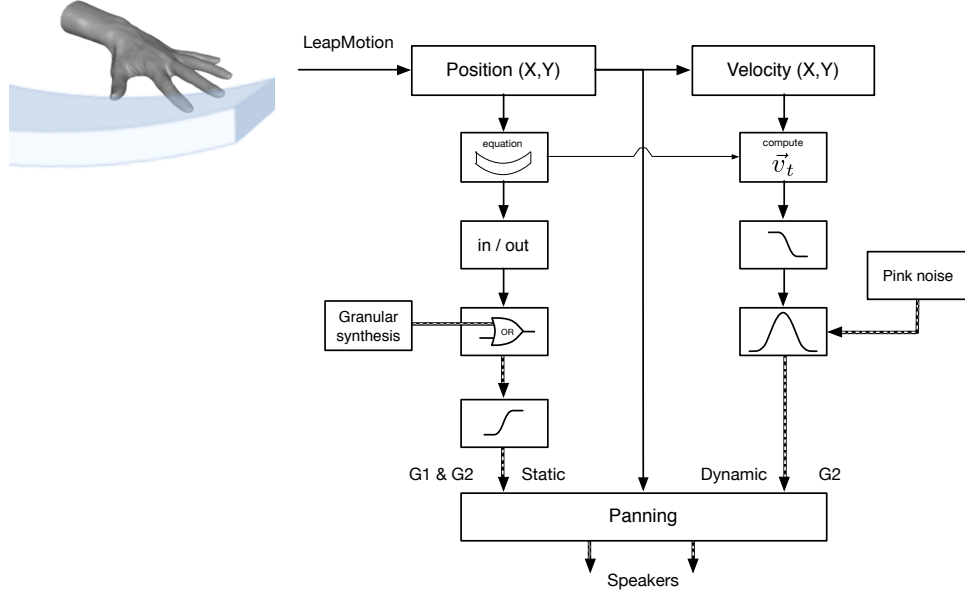
Figure 4.4 – Schematic of the static and dynamic sonification processes.
