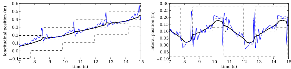
Figure 6.10.: Detailed ZMP tracking performance. From left to right — longitudinal direction, lateral direction. Thin solid blue: measured CoP position — thick solid black: CoM position — dotted blue: ZMP reference — dashed black: actual BoS boundaries.
