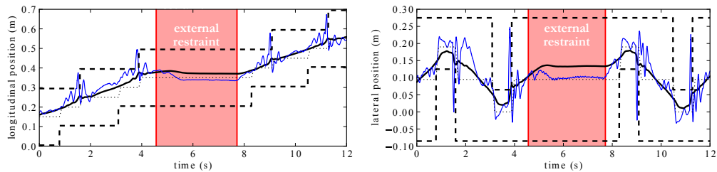
Figure 6.16.: Detail of the evolution of the CoP against the external restraint. From left to right — longitudinal direction, lateral direction. Thin solid blue: measured CoP position — thick solid black: CoM position — dotted blue: ZMP reference — dashed black: actual BoS boundaries.
