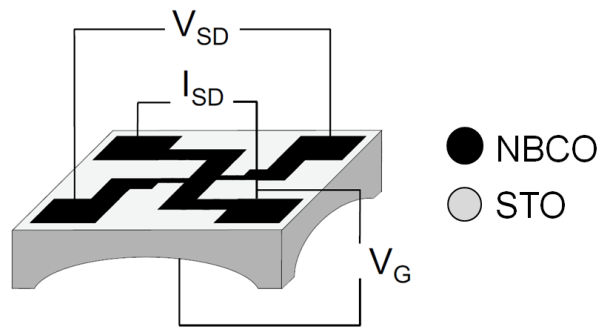
Figure II.3: Field-Effect transistor. STO is mild down to 100 \text{ }\mu\text{m} and coated with gold. V_G : gate voltage; I_{SD} and V_{SD} : current and voltage from the source to the drain. Taken from [107]
