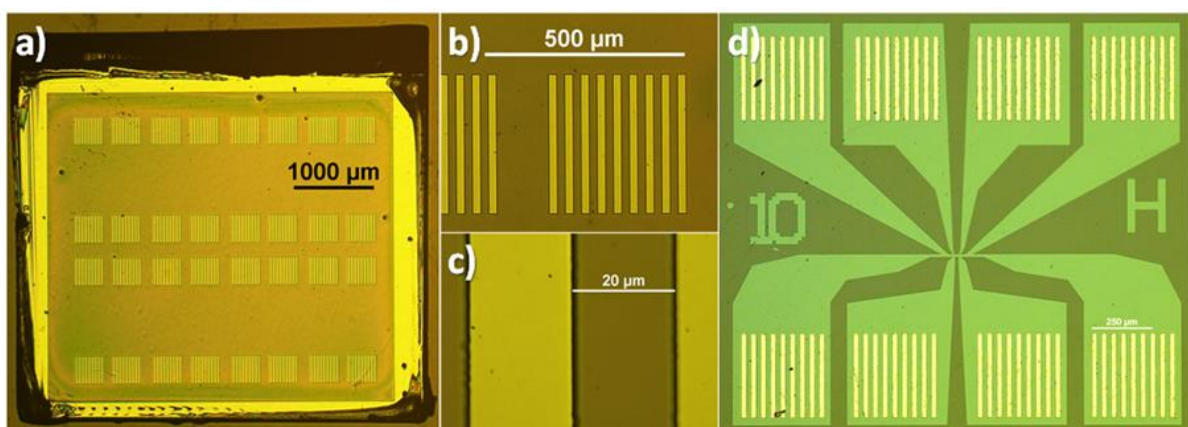
Figure III.18: Pictures of a 5x5 mm 2 devices after designing the contact stripes a) x1, b) x5 and c) x100 and d) after designing the bridge
