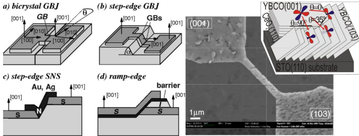
Figure I.12: Left: types of high- T_c Josephson junctions, taken from [44]; Right: SEM image of a 0.8 \mu\text{m} wide biepitaxial junction. The inset sketches the junction's structure. Taken from [45]
