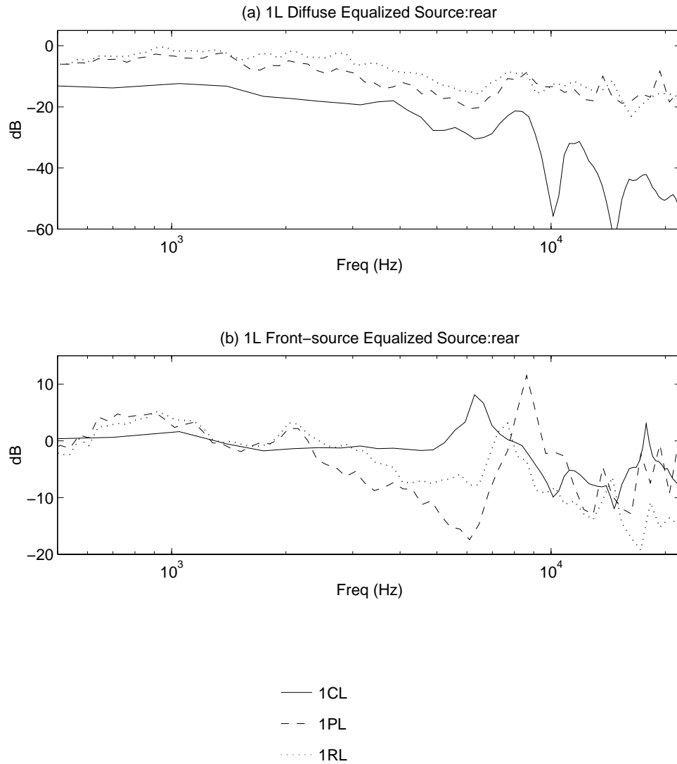
Figure 4.29: Experimentally measured HRTF for source rear with data sets 1L for each experimental and equalization method. Sources were 1CL : 4, 1PL : 18, and 1RL : 18.
