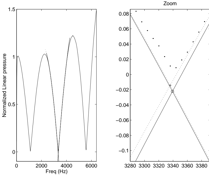
Figure 3.5: Results of interpolation to determine precise frequency null, and consequent microphone position. The dotted line(+) indicate the first pass interpolation and the solid line(o) indicate the final interpolation result.
