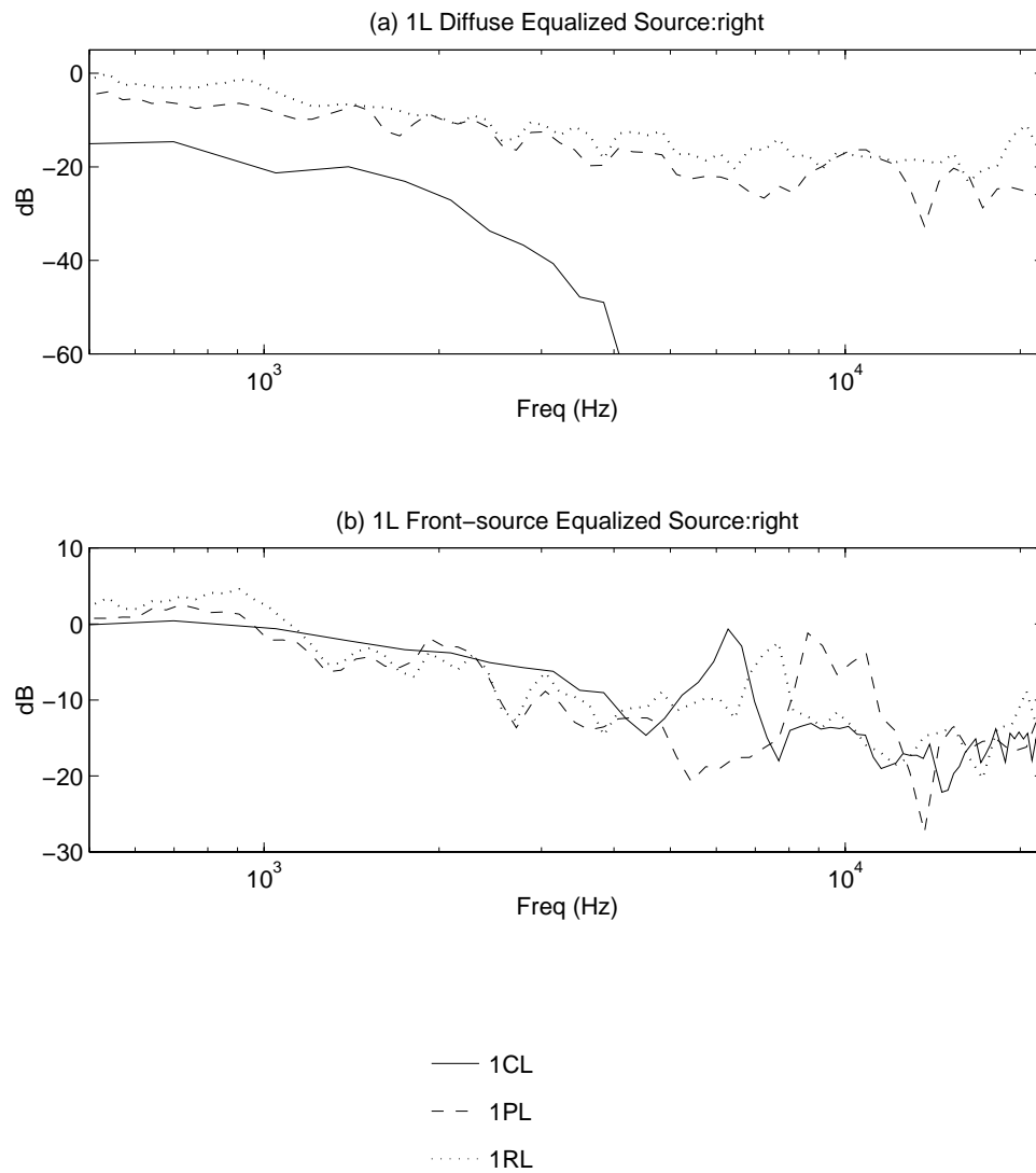
Figure 4.28: Experimentally measured HRTF for source right with data sets 1L for each experimental and equalization method. Sources were 1CL : 58, 1PL : 12, and 1RL : 12.
