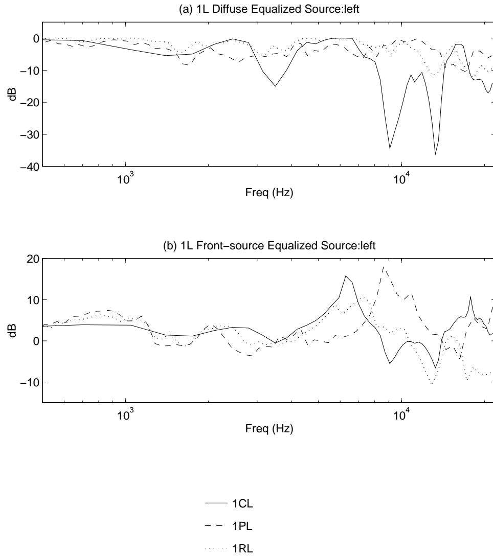
Figure 4.27: Experimentally measured HRTF for source left with data sets 1L for each experimental and equalization method. Sources were 1CL : 22 , 1PL : 1 , and 1RL : 1 .
