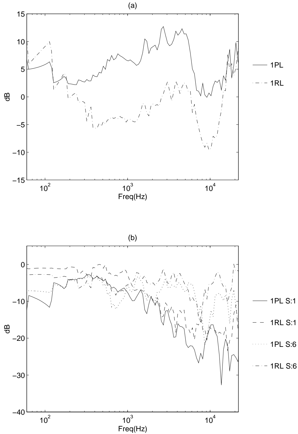
Figure 4.3: Diffuse field equalization examples. (a) Diffuse field equalization functions for 1PL and 1RL. (b) Diffuse field equalized data showing sources front (WPAFB Source:6) and right (WPAFB Source:1) for 1L.
