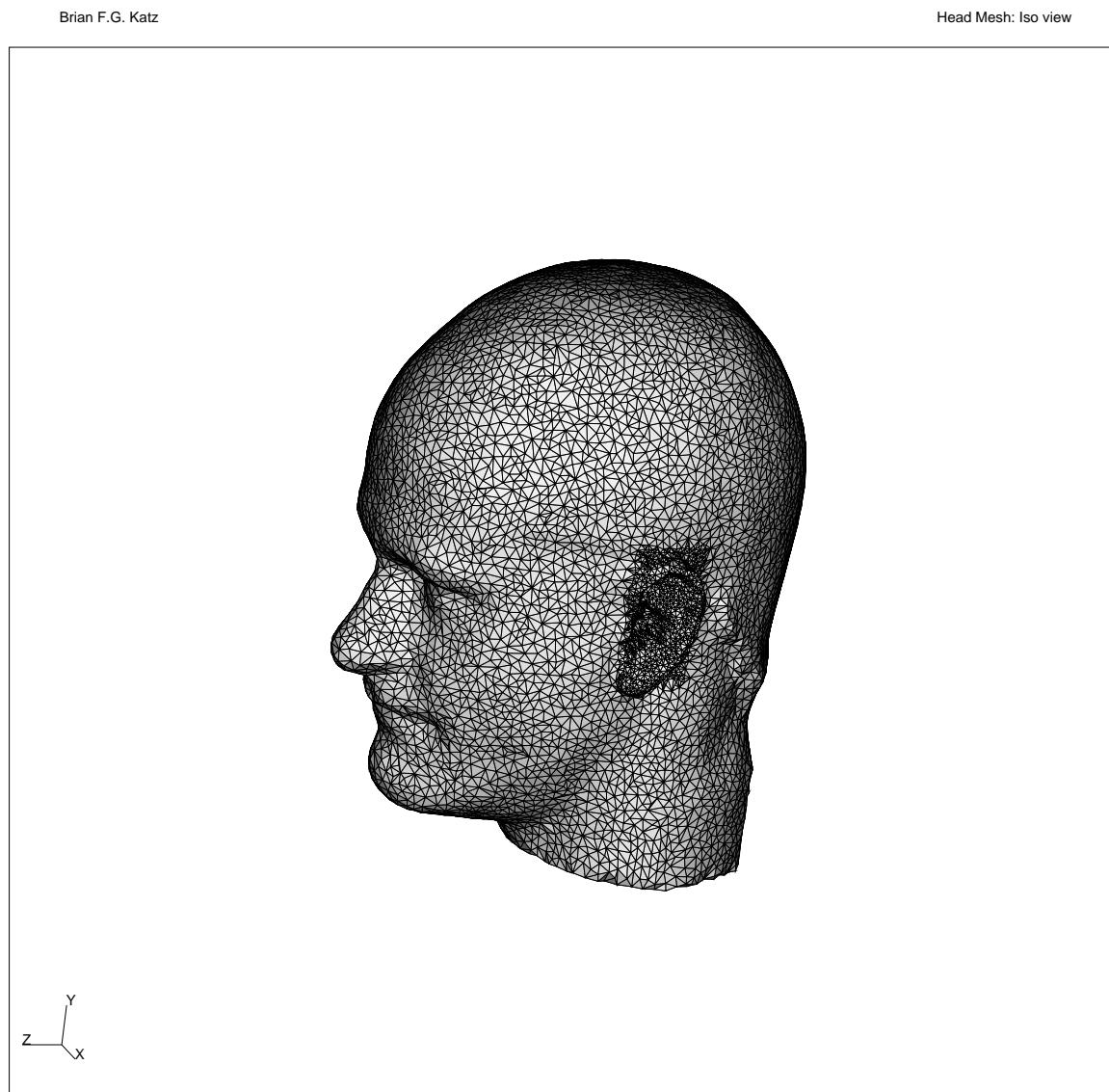
Figure 5.6: The full BEM mesh used. Frequency limitation of 5.4 kHz for 4 nodes/wavelength. Note the increased resolution in the pinna region. Isometric view.
