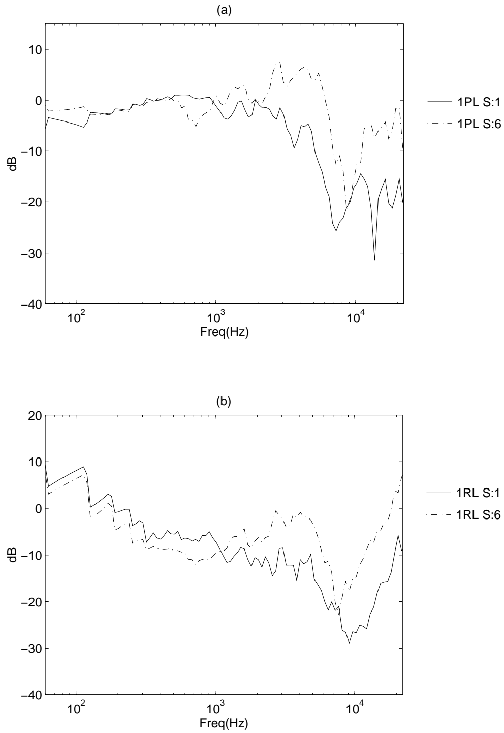
Figure 4.2: Free field equalized data showing sources front (WPAFB Source:6) and right(WPAFB Source:1) for (a) 1PL and (b) 1RL.
