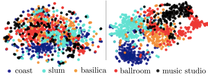
Figure 4.2 – t-distributed Stochastic Neighbor Embedding (t-SNE) visualization on Cross-Modal Places (CMPlaces) sentences for a set of randomly sampled visual scenes. Left: textual model \mathbf{T} . Right: grounded model \mathbf{C}_g + \mathbf{P}_g .
