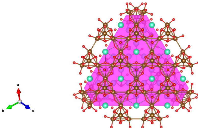
Figure 1.13: Lu_2V_2O_7 crystal structure projected in \langle 111 \rangle (shown as the pink plane), where the element of Lu, V, O are represented by the color bull of aqua, coffee and red, respectively.
